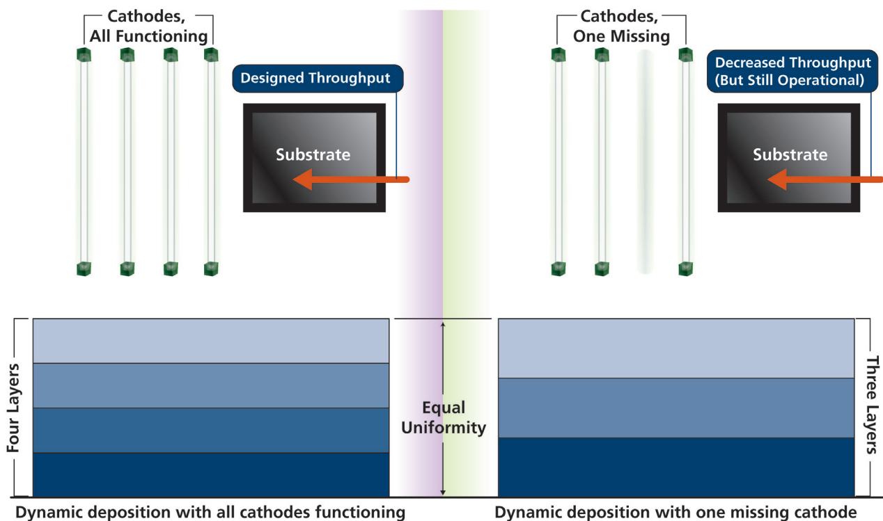
Figure 1. Dynamic system with one missing cathode—the system runs more slowly and creates three layers instead of four, but maintains overall uniformity. Therefore, production can continue, although at a slower rate
