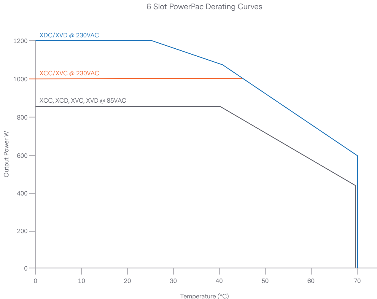
Figure 3: Thermal derating of the Xgen series
