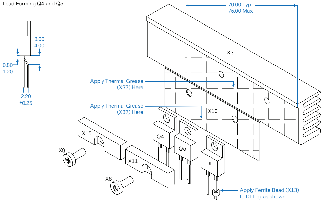
Figure 2: A combination of conduction and convection cooling provide effective thermal management
