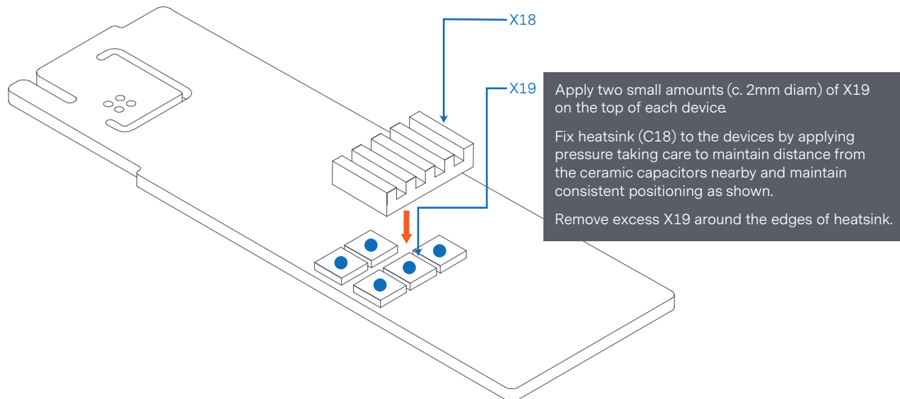
Figure 1: Heatsinks used to keep key components running at a lower temperature
