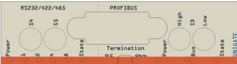
Picture 2: Front panel: Rotary switches and LEDs
