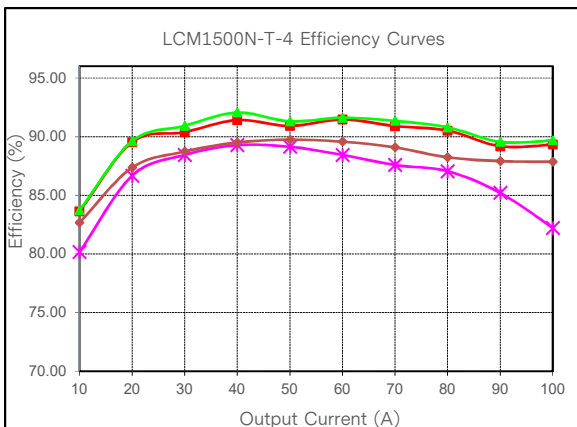
Figure 20: LCM1500N-T-4 Efficiency Curve @ 25°C — 90Vac — 115Vac — 230Vac — 264Vac Loading: I_{o\_main} = 10\%I_{o\_max} increment to 100A, I_{sb} = 0A (5V)
