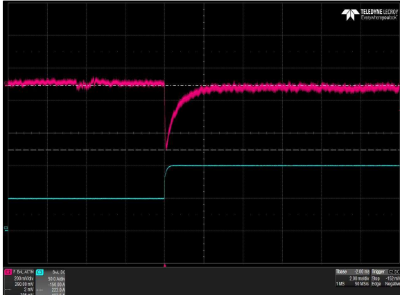
Figure 18: LCM1500N-T-4 Transient Response - Vo Deviation 50% to 100% load change 1A/uS slew rate Vin = 230Vac Ch 1: Vo Ch 2: Io
