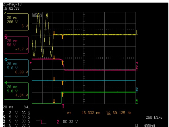
Figure 59: LCM1500W-T-4 Hold-up Time Vin = 264Vac / 60Hz / 0° Load: Io = 32A (48V), Isb = 2A (5V) Ch 1: Vin Ch 2: Vsb Ch 3: Vo Ch 4: G_DCOK_C
