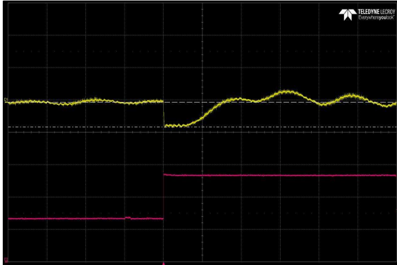
Figure 40: LCM1500R-T-4 Transient Response - Vo Deviation 50% to 100% load change 1A/uS slew rate Vin = 230Vac Ch 1: Vo Ch 2: Io
