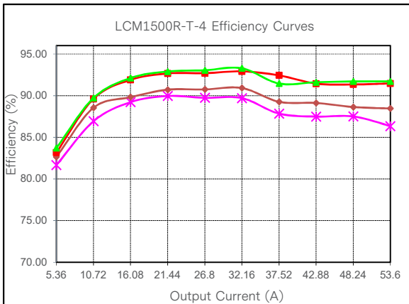
Figure 42: LCM1500R-T-4 Efficiency Curve @ 25°C Loading: I_{o\_main} = 10\%I_{o\_max} increment to 53.6A, I_{SB} = 0A (5V) — 90Vac — 115Vac — 230Vac — 264Vac
