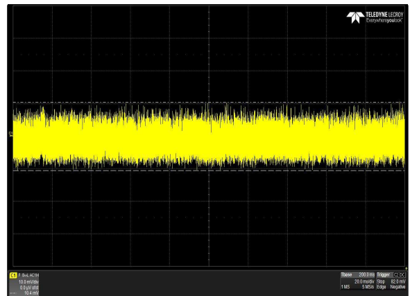
Figure 21: LCM1500N-T-4 Ripple and Noise Measurement Vin = 115Vac Load: Io = 100A (15V), Isb = 2A (5V) Ch 1: Vo
