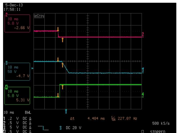
Figure 61: LCM1500W-T-4 Turn Off Characteristic via INH_EN Load: Io = 32A (48V), Isb = 2A (5V) Ch 2: INH_EN Ch 3: Vo Ch 4: G_DCOK_C
