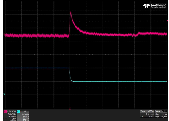
Figure 19: LCM1500N-T-4 Transient Response - Vo Deviation 100% to 50% load change 1A/uS slew rate Vin = 230Vac Ch 1: Vo Ch 2: Io
