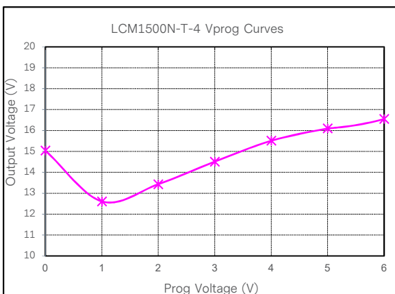
Figure 22: LCM1500N-T-4 Output Voltage Adjustment by Vprog @ 25°C — 115Vac Loading: I_o = 0A (15V), I_{sb} = 0A (5V)
