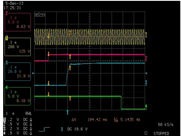
Figure 57: LCM1500W-T-4 Turn-on delay via INH_EN Vin = 90Vac Load: Io = 32A (48V), Isb = 2A (5V) Ch 1: Vin Ch 2: INH_EN Ch 3: Vo Ch 4: G_DCOK_C
