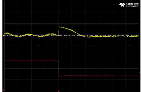
Figure 41: LCM1500R-T-4 Transient Response - Vo Deviation 100% to 50% load change 1A/uS slew rate Vin = 230Vac Ch 1: Vo Ch 2: Io
