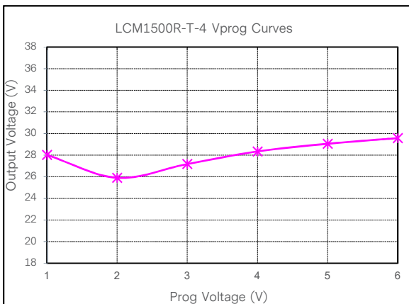
Figure 44: LCM1500R-T-4 Output Voltage Adjustment by Vprog @ 25°C Loading: I_o = 0A (28V), I_{SB} = 0A (5V) — 115Vac
