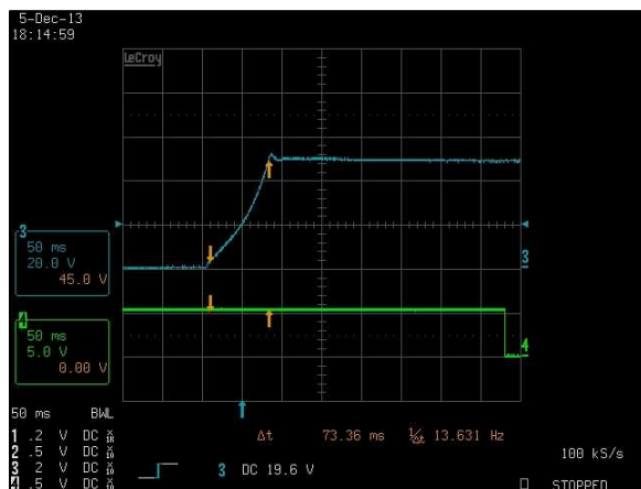
Figure 60: LCM1500W-T-4 Output Voltage Startup Vin = 90Vac Load: Io = 32A (48V), Isb = 2A (5V) Ch 3: Vo Ch 4: G_DCOK_C
