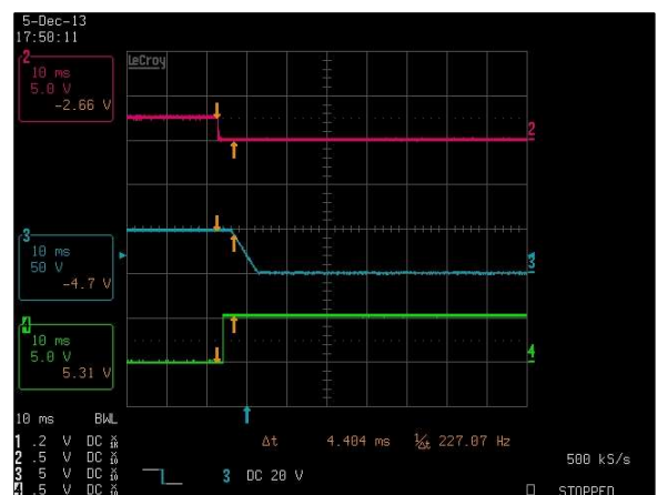
Figure 50: LCM1500U-T-4 Turn Off Characteristic via INH_EN Load: Io = 42A (36V), Isb = 2A (5V) Ch 2: INH_EN Ch 3: Vo Ch 4: G_DCOK_C
