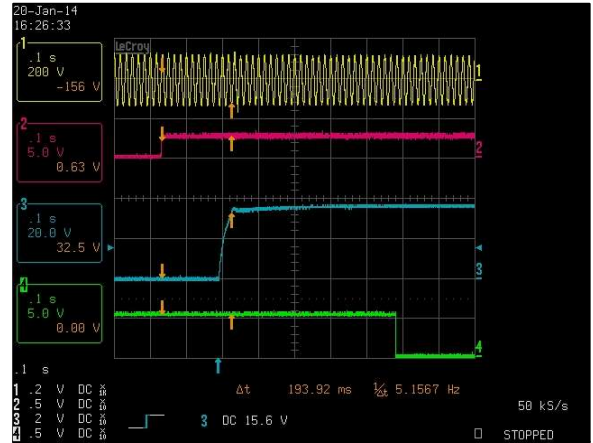
Figure 46: LCM1500U-T-4 Turn-on delay via INH_EN Vin = 90Vac Load: Io = 42A (36V), Isb = 2A (5V) Ch 1: Vin Ch 2: INH_EN Ch 3: Vo Ch 4: G_DCOK_C
