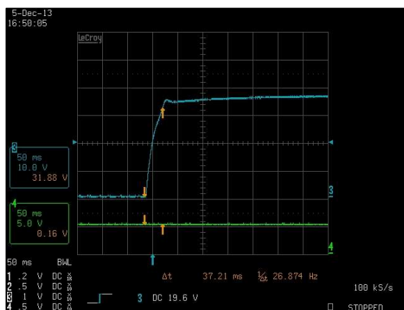
Figure 49: LCM1500U-T-4 Output Voltage Startup Vin = 90Vac Load: Io = 42A (36V), Isb = 2A (5V) Ch 3: Vo Ch 4: G_DCOK_C
