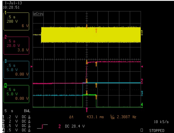
Figure 45: LCM1500U-T-4 Turn-on delay via AC mains Vin = 90Vac Load: Io = 42A (36V), Isb = 2A (5V) Ch 1: Vin Ch 2: Vsb Ch 3: Vo Ch 4: G_DCOK_C
