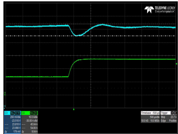
Figure 20: CNS655-MU Transient Response – V_o Deviation V_{IN} = 90\text{Vac} , I_O = 100\% to 50%, Output Cap = 330 \mu\text{F} /A Ch 3: V_o Ch 4: I_O
