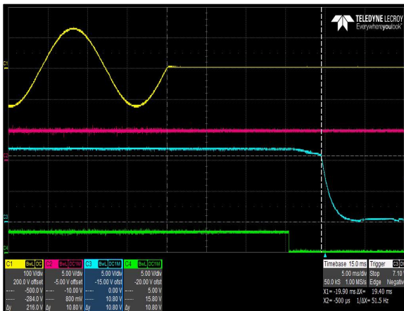
Figure 3: CNS653-ME Hold-up Time – V_{IN} = 90\text{Vac} / 63\text{Hz} / 0^\circ Load: I_O = 54.2\text{A} , I_{SB} = 2\text{A}
