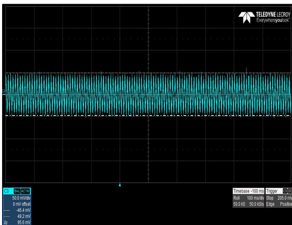
Figure 21: CNS655-MU Ripple and Noise Measurement V_{in} = 115\text{Vac} , Load: I_O = 16.7\text{A} Ch 3: V_o
