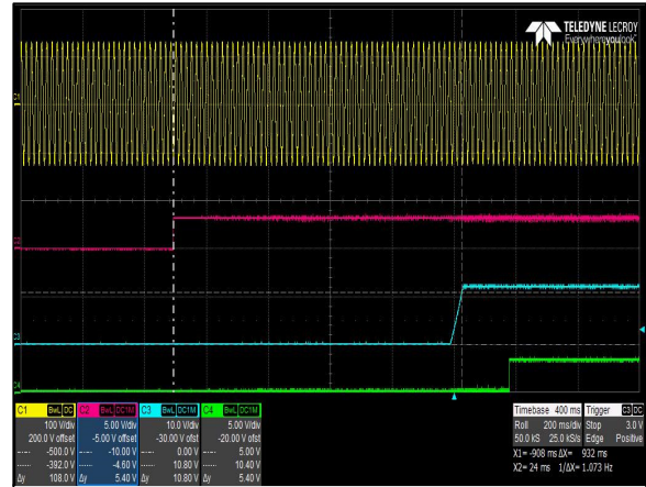
Figure 2: CNS653-ME Turn-on delay by Inhibit – V_{IN} = 90\text{Vac} Load: I_O = 54.2\text{A} , I_{SB} = 2\text{A}
