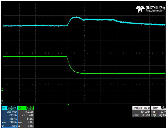
Figure 19: CNS655-MU Transient Response – V_o Deviation V_{IN} = 90\text{Vac} , I_O = 100\% to 50%, Output Cap = 330 \mu\text{F} /A Ch 3: V_o Ch 4: I_O
