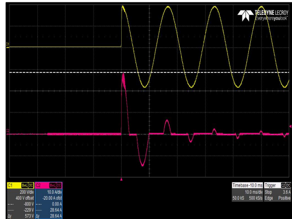
Figure 6: CNS653-ME Inrush Current V_{IN} = 264\text{Vac} , Load: I_O = 0\text{A} , Turn on angle = 90^\circ
