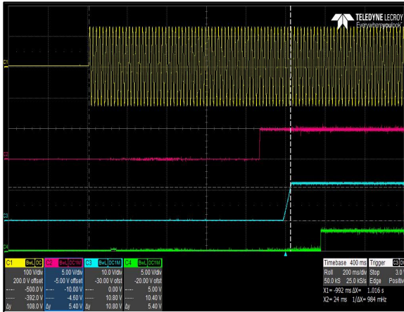
Figure 1: CNS653-ME Turn-on delay by AC Mains – V_{IN} = 90\text{Vac} Load: I_O = 54.2\text{A} , I_{SB} = 2\text{A}
