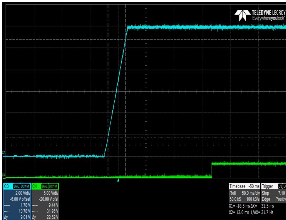
Figure 5: CNS653-ME Output Voltage Startup Characteristic V_{IN} = 90\text{Vac} , Load: I_O = 54.2\text{A}
