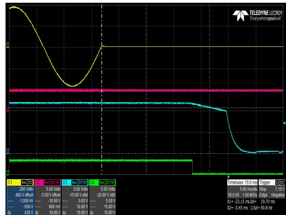
Figure 4: CNS653-ME Hold-up Time – V_{IN} = 264\text{Vac} / 47\text{Hz} / 0^\circ Load: I_O = 54.2\text{A} , I_{SB} = 2\text{A}
