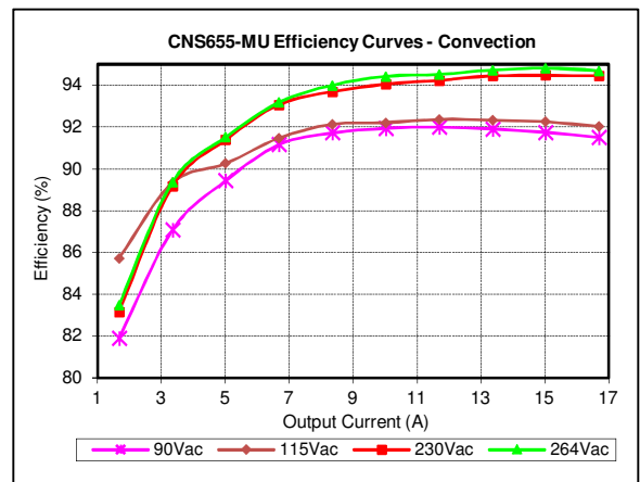
Figure 22: CNS655-MU Efficiency Curves @ 25°C Convection Cooling V_{IN} = 90 to 264Vac, Load: I_O = 0 to 16.7A
