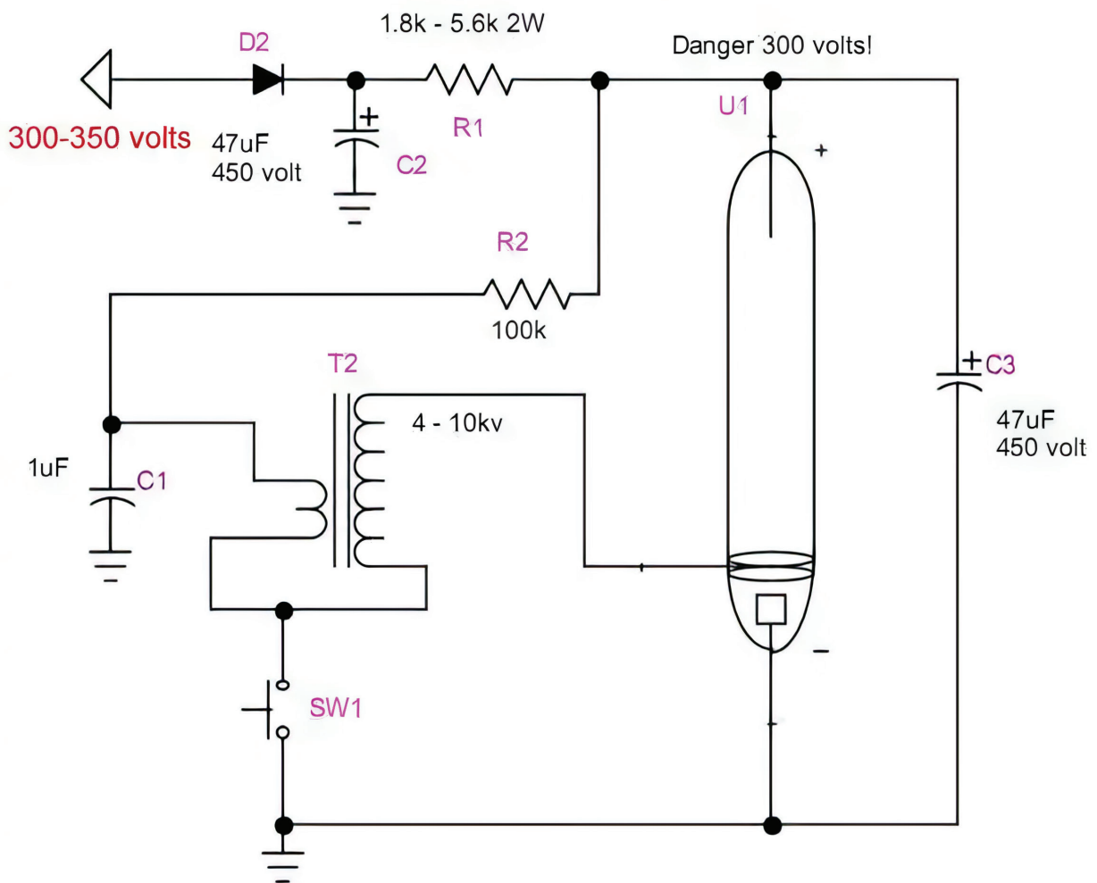
Figure 3. Flashlamp Circuit
