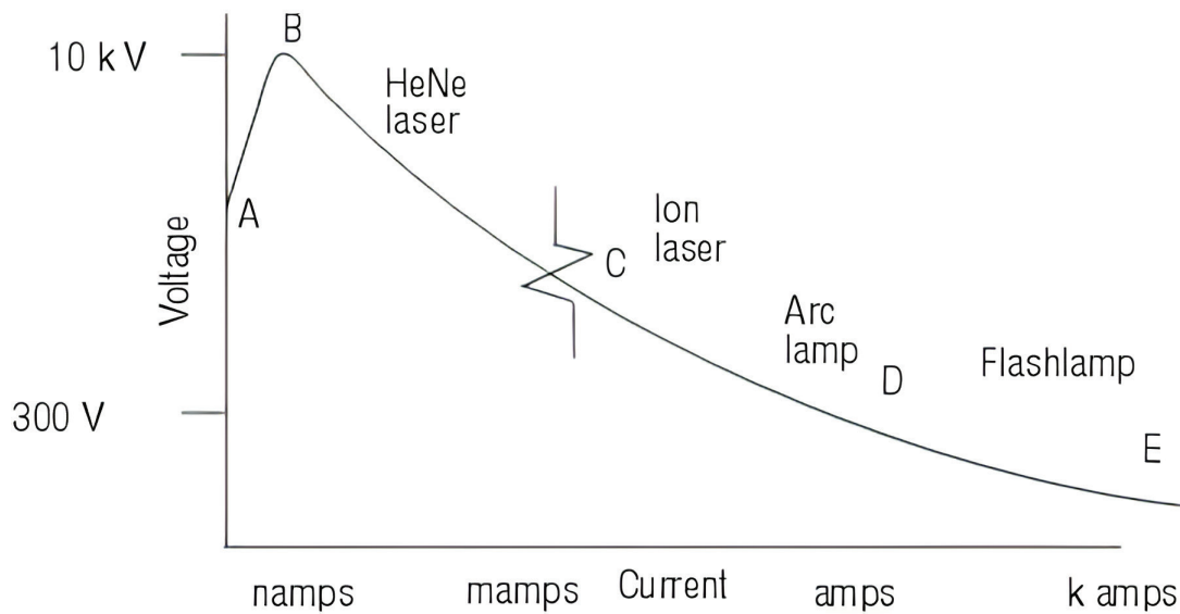
Figure 2. Current/Voltage Curve for Gas Discharge Lasers
