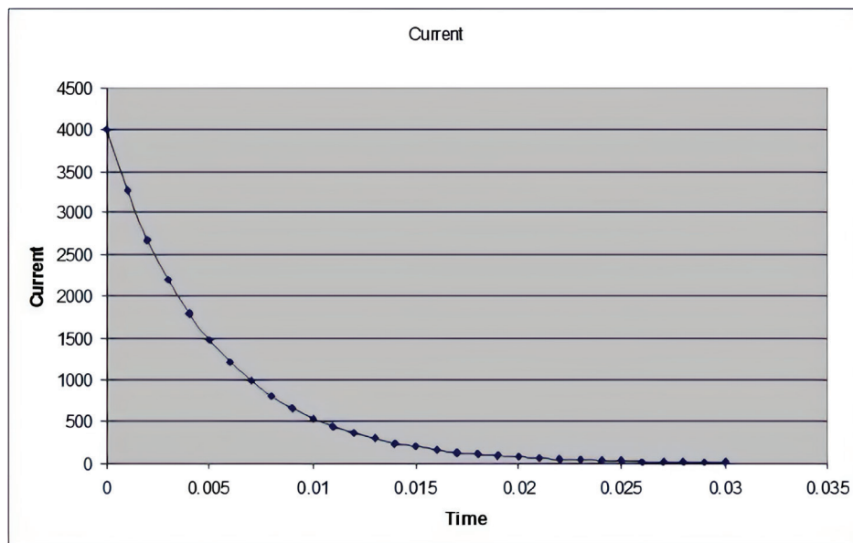
Figure 4. Charging Capacitance with Constant Voltage
