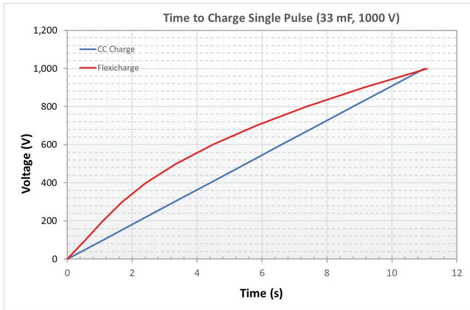
Figure 5. Charging Capacitance with a Constant Current and Constant Power
