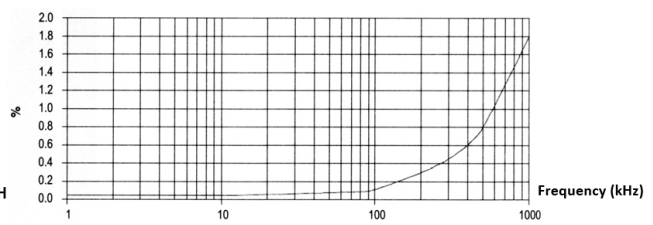
Figure 4: Distortion (Typical) 4
