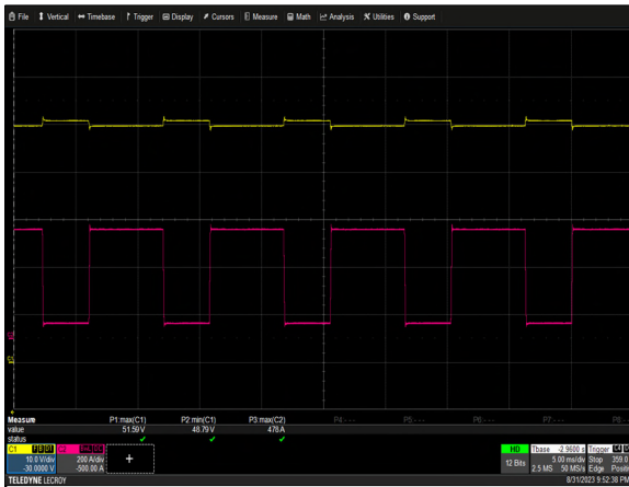
Figure 13: ORV3 Shelf Pulse Load (6 PSUs in the shelf) Vin = 400Vac(L-L) Io = 60A(3.75ms) to 450A (6ms) repetitive Ch 1:Vo Ch 2: Io (slow rate: 5A/us)
