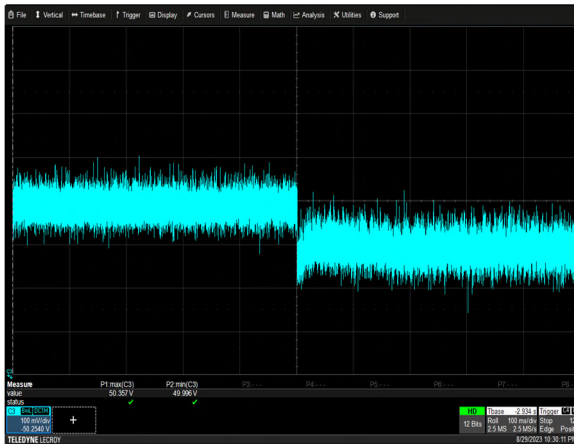
Figure 23: ORV3 Hot Swap Peak Deviation (Extract the 6th PSU) Vin = 400Vac (L-L) Io = 300A Ch 3: Vo (100mV/div, 100ms/div)
