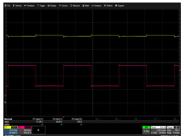
Figure 18: ORV3 Shelf Pulse Load (5 PSUs in the shelf) Vin = 400Vac(L-L) Io = 150A(8ms) to 450A (8ms) repetitive Ch 1:Vo Ch 2: Io (slow rate: 5A/us)
