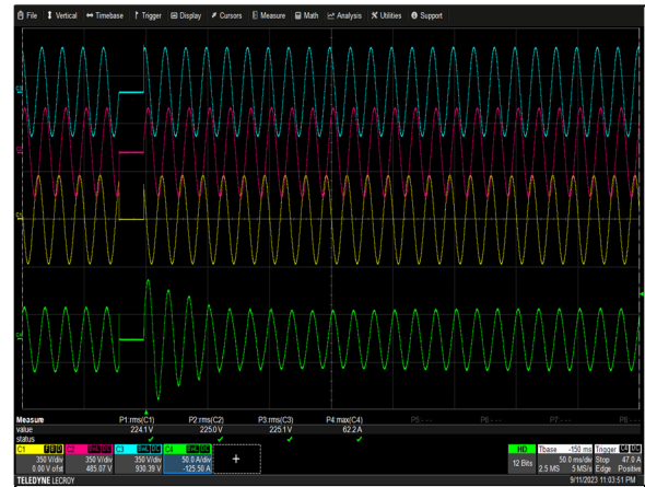
Figure 20: ORV3 Shelf Inrush Current Vin = 230Vac(L-N) (3 phases drop for 20ms) Io = 300A Ch 1: Vin (L1-N) Ch 2: Vin (L2-N) Ch 3: Vin (L3-N) Ch 4: Iin
