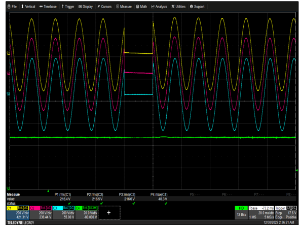
Figure 8: ORV3 Shelf Ride Through Test (5 PSUs in the shelf) Vin = 230Vac to 0V (20ms) to 230Vac (L-N) Io = 300A Ch 1: Vin (L1-N) Ch 2: Vin (L2-N) Ch3: Vin (L3-N) Ch4:Vo
