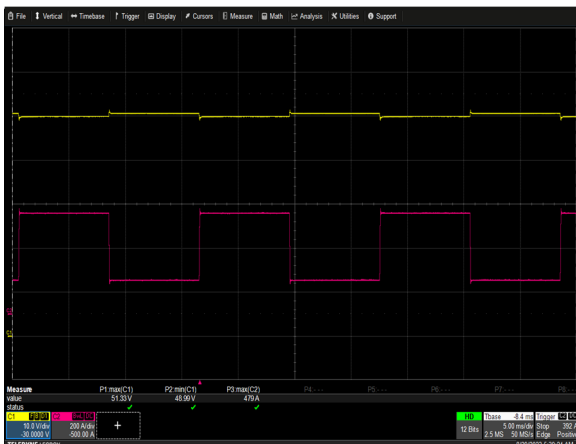
Figure 17: ORV3 Shelf Pulse Load (6 PSUs in the shelf) Vin = 400Vac(L-L) Io = 150A(8ms) to 450A (8ms) repetitive Ch 1:Vo Ch 2: Io (slow rate: 5A/us)
