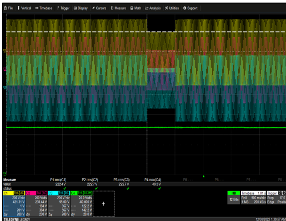
Figure 9: ORV3 Shelf Ride Through Test (6 PSUs in the shelf) Vin = 230Vac to 140V (500ms) to 230Vac (L-N) Io = 300A Ch 1: Vin (L1-N) Ch 2: Vin (L2-N) Ch3: Vin (L3-N) Ch4:Vo
