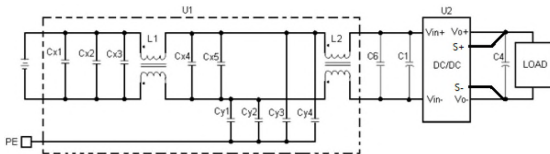
Figure 20 EMC test configuration
