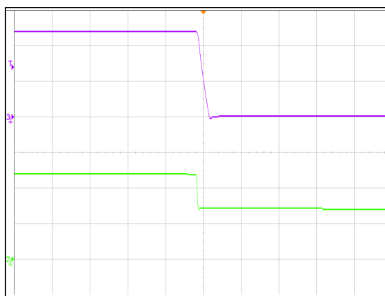
Figure 4: ADQ600B-48S12B Turn Off Characteristic (5mS/div) V_{in} = 48V_{dc} Load: I_o = 50A Ch 2: V_i (20V/div) Ch 3: V_o (5V/div)
