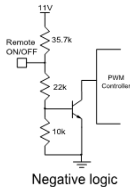
Figure 16 Remote ON/OFF internal diagram
