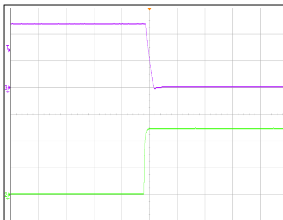
Figure 6: ADQ600B-48S12B Remote OFF Waveform (5mS/div) V_{in} = 48V_{dc} Load: I_o = 50A Ch 2: Remote OFF (2V/div) CH3: V_o (5V/div)
