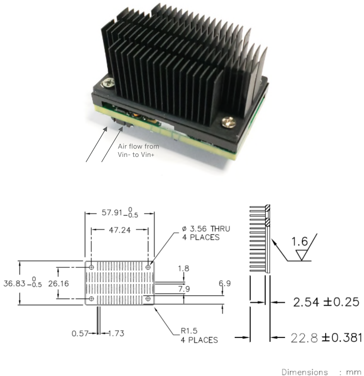
Figure 13 Typical test condition, heatsink
