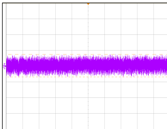
Figure 2: ADQ600B-48S12B Ripple and Noise Measurement V_{in} = 48V_{dc} Load: I_o = 50A Ch 3: V_o (1ms/div, 50mV/div)
