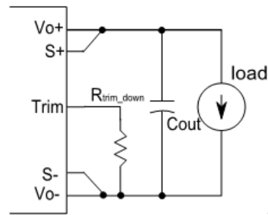
Figure 18 Trim down
