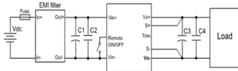
Figure 15 Typical application
