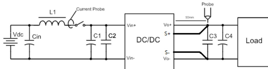
Figure 19 Input ripple &amp; inrush current output ripple &amp; noise test configuration
