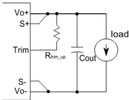
Figure 17 Trim up
