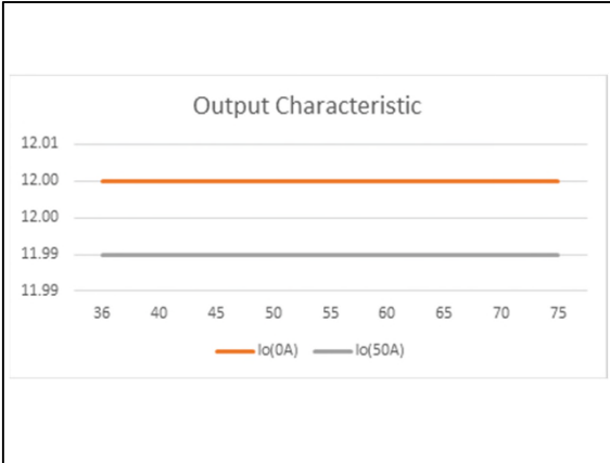
Figure 10: ADQ600B-48S12B Output Characteristic Loading: Io=0~50A
