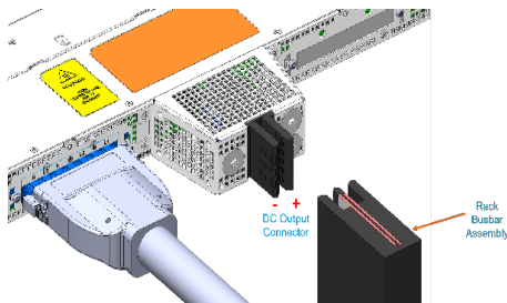
1AC DC Output Connector
