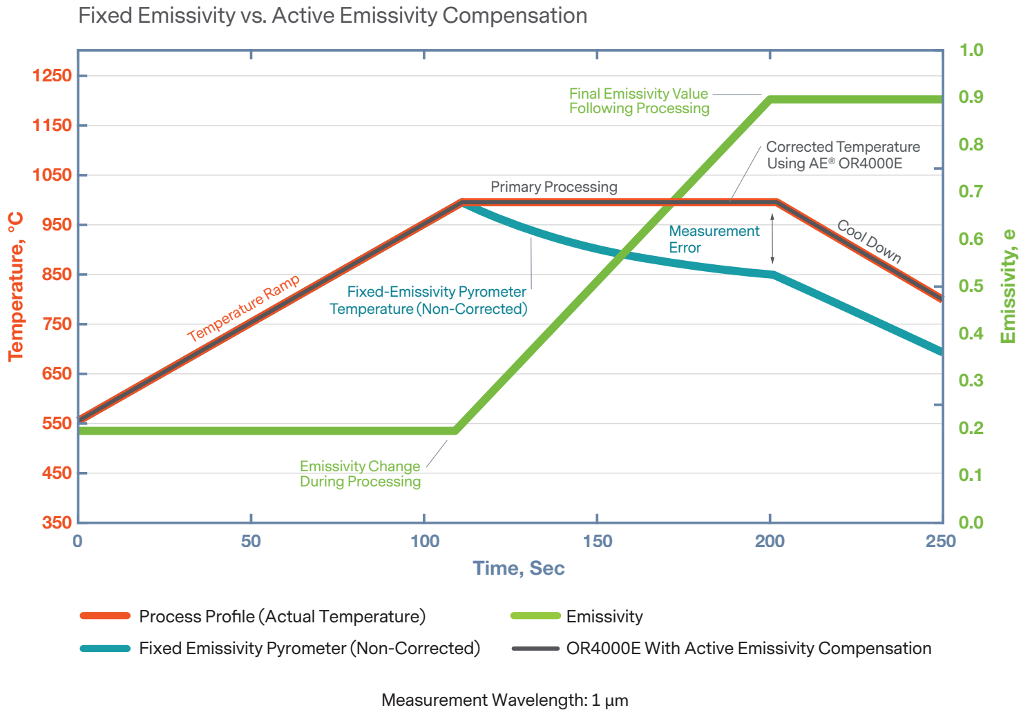
Figure 3. Temperature measurement accuracy for an object with changing emissivity: fixed emissivity vs. active emissivity compensation
