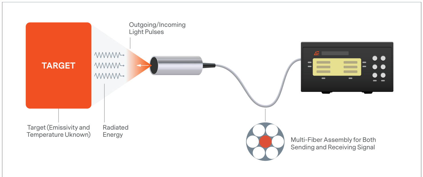
Figure 4. Measuring emissivity
