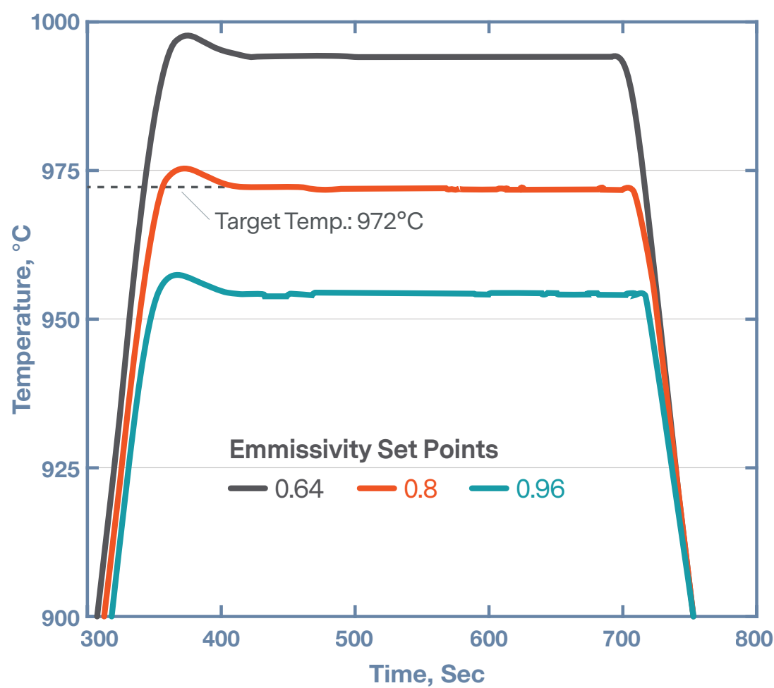
Figure 2. Temperature measurement using fixed emissivity
