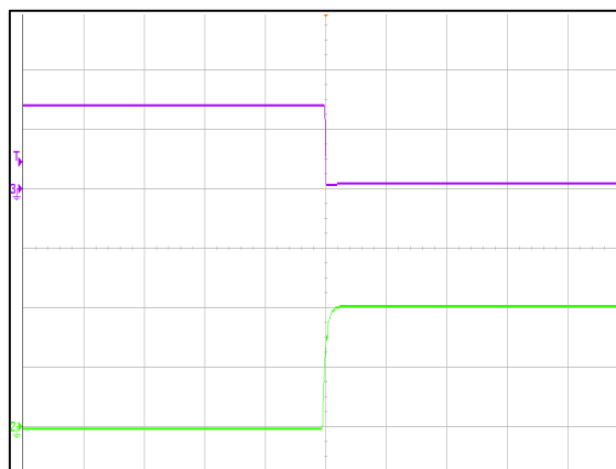
Figure 6: ADH1300-48S28B Transient Response (2mS/div) V_{in} = 48V_{dc} Load: I_o = 46.5A (50mS/div) Ch 2: Remote OFF (2V/div) Ch 3: V_o (20V/div)
