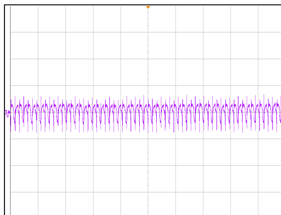
Figure 2: ADH1300-48S28B Ripple and Noise Measurement V_{in} = 48V_{dc} Load: I_o = 46.5A Ch 3: V_o (20us/div, 100mV/div)
