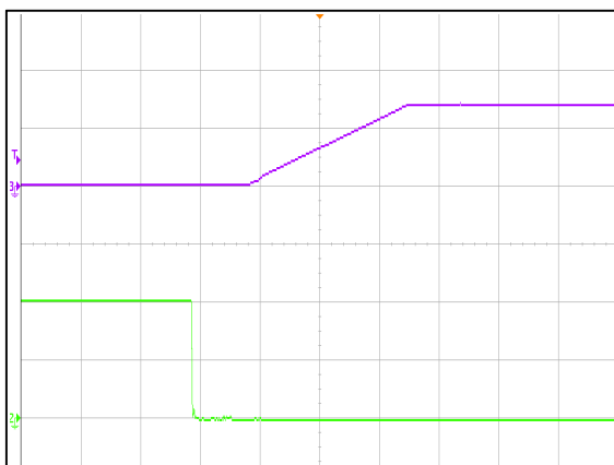
Figure 5: ADH1300-48S28B Remote ON Waveform V_{in} = 48V_{dc} Load: I_o = 46.5A (50mS/div) Ch 2: Remote ON (2V/div) Ch 3: V_o (20V/div)
