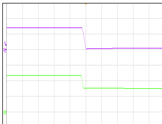
Figure 4: ADH1300-48S28B Turn Off Characteristic V_{in} = 48V_{dc} Load: I_o = 46.5A Ch 2: V_i (20V/div) Ch 3: V_o (20V/div)
