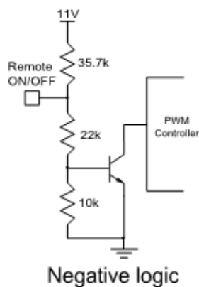
Figure 15 External Remote ON/OFF circuit
