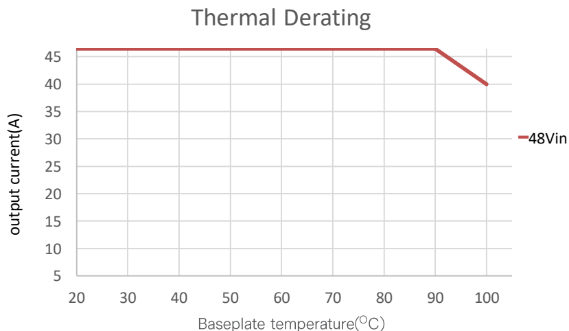
Figure 13 Available load current vs Base plate temperature
