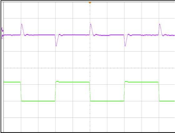
Figure 7: ADH1300-48S28B Transient Response (2mS/div) Vin = 48Vdc Io = 50%~75%~50% load change, 0.1A/ \mu S slew rate Ch 2: Io (10A/div) Ch 3: Vo (500mV/div)
