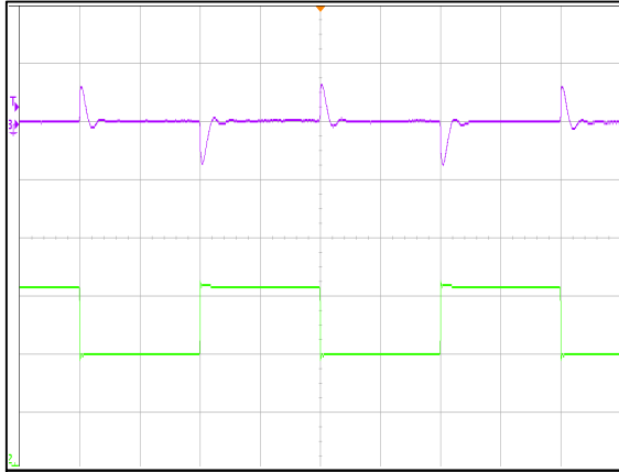
Figure 8: ADH1300-48S28B Transient Response (2mS/div) Vin = 48Vdc Io = 25%~50%~25% load change, 0.1A/ \mu S slew rate Ch 2: Io (10A/div) Ch 3: Vo (500mV/div)
