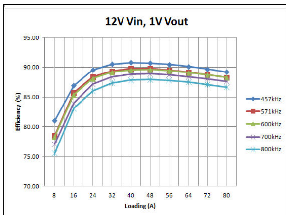
Figure 6: LGA80D-00DADJJ Efficiency Curves @ 25°C, 200LFM
