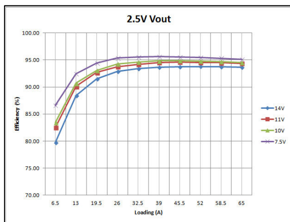
Figure 3: LGA80D-00DADJJ Efficiency Curves @ 25°C, 200LFM
