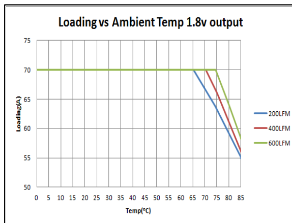
Figure 12: LGA80D-00DADJJ Thermal Derating Curves (Two modules with longitudinal airflow) Vin = 12V Load: Io = 50 to 70A, Vo = 1.8V Fsw = 457kHz
