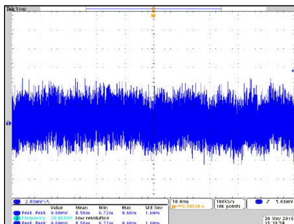
Figure 17: LGA80D-00DADJJ Ripple and Noise - V_o = 1.0V
