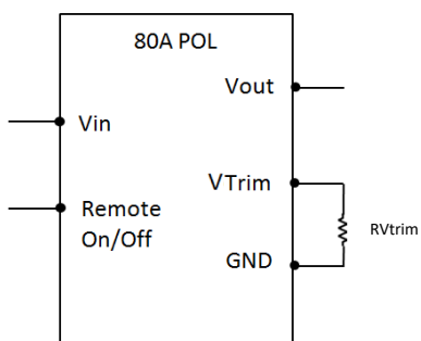
Figure 41: Output Voltage Adjustment
