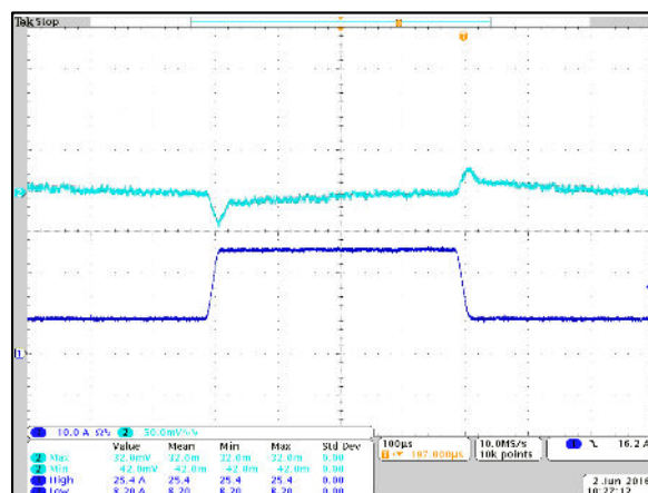
Figure 30: LGA80D-00DADJJ Transient Response - Vo Deviation 25% to 75% to 25% load, 1A/µs slew rate, Vin = 12Vdc, Vo = 2.5V Ch 1: Io Ch 2: Vo
