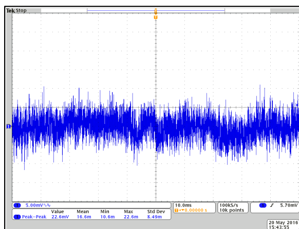
Figure 21: LGA80D-00DADJJ Ripple and Noise - V_o = 5.0V
