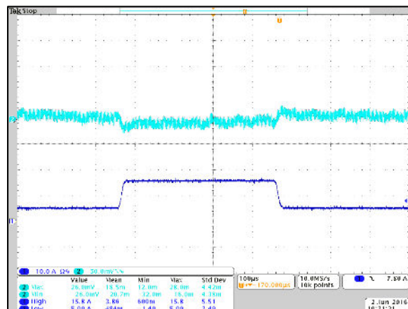
Figure 32: LGA80D-00DADJJ Transient Response - Vo Deviation 25% to 75% to 25% load, 1A/µs slew rate, Vin = 12Vdc, Vo = 5.0V Ch 1: Io Ch 2: Vo
