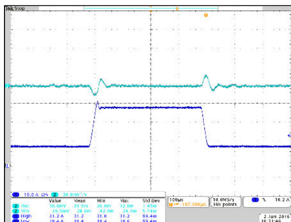
Figure 27: LGA80D-00DADJJ Transient Response - Vo Deviation 25% to 75% to 25% load, 1A/µs slew rate, Vin = 12Vdc, Vo = 0.6V Ch 1: Io Ch 2: Vo
