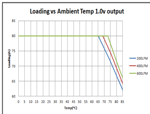
Figure 11: LGA80D-00DADJJ Thermal Derating Curves (Two modules with longitudinal airflow) Vin = 12V Load: Io = 60 to 80A, Vo = 1.0V Fsw = 457kHz
