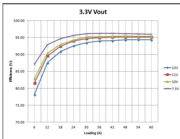
Figure 4: LGA80D-00DADJJ Efficiency Curves @ 25°C, 200LFM
