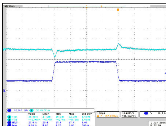
Figure 29: LGA80D-00DADJJ Transient Response - Vo Deviation 25% to 75% to 25% load, 1A/µs slew rate, Vin = 12Vdc, Vo = 1.8V Ch 1: Io Ch 2: Vo
