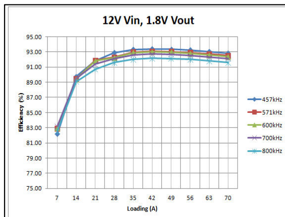
Figure 7: LGA80D-00DADJJ Efficiency Curves @ 25°C, 200LFM
