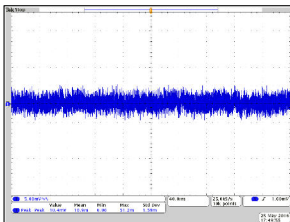
Figure 18: LGA80D-00DADJJ Ripple and Noise - V_o = 1.8V
