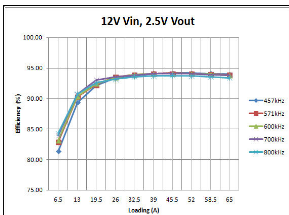
Figure 8: LGA80D-00DADJJ Efficiency Curves @ 25°C, 200LFM
