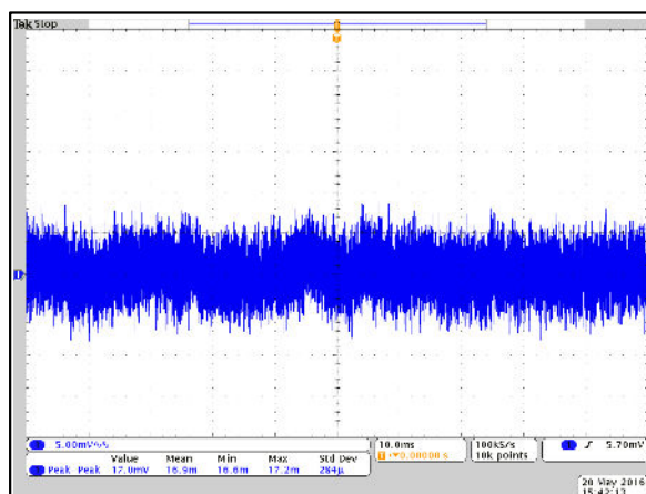
Figure 19: LGA80D-00DADJJ Ripple and Noise - V_o = 2.5V
