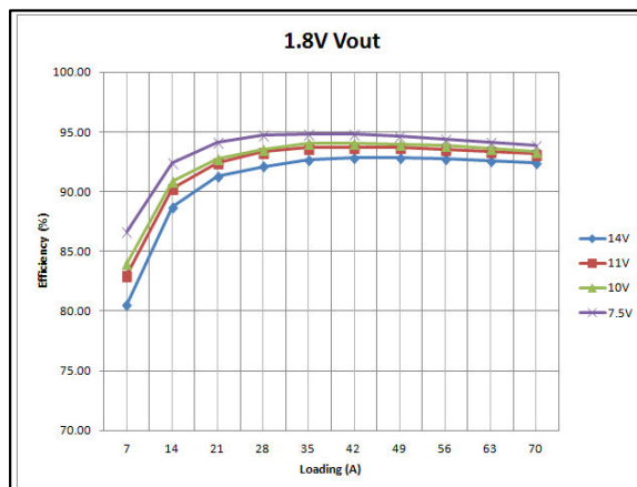
Figure 2: LGA80D-00DADJJ Efficiency Curves @ 25°C, 200LFM
