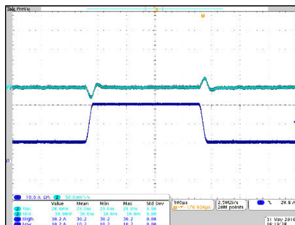
Figure 28: LGA80D-00DADJJ Transient Response - Vo Deviation 25% to 75% to 25% load, 1A/µs slew rate, Vin = 12Vdc, Vo = 1.0V Ch 1: Io Ch 2: Vo
