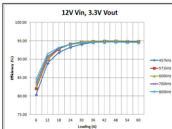
Figure 9: LGA80D-00DADJJ Efficiency Curves @ 25°C, 200LFM
