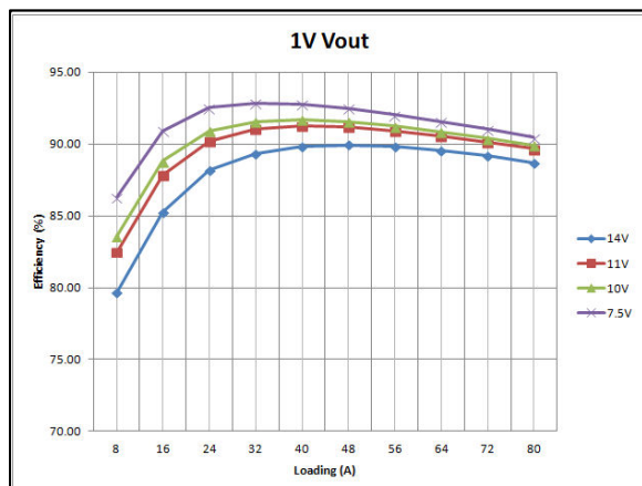
Figure 1: LGA80D-00DADJJ Efficiency Curves @ 25°C, 200LFM
