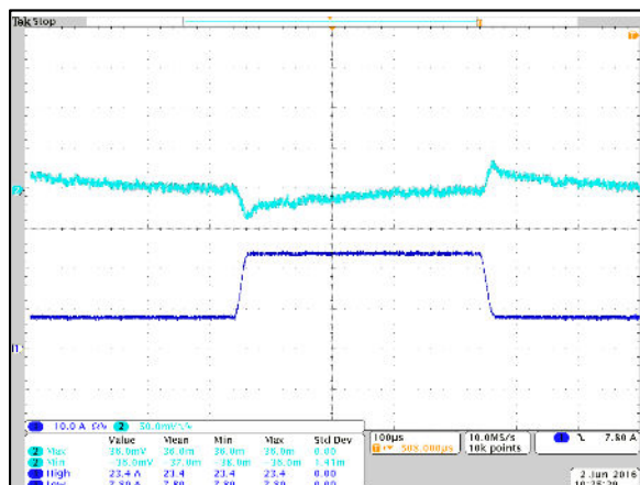
Figure 31: LGA80D-00DADJJ Transient Response - Vo Deviation 25% to 75% to 25% load, 1A/µs slew rate, Vin = 12Vdc, Vo = 3.3V Ch 1: Io Ch 2: Vo
