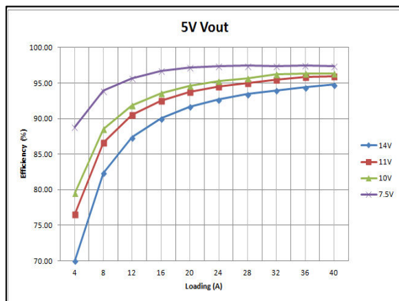
Figure 5: LGA80D-00DADJJ Efficiency Curves @ 25°C, 200LFM
