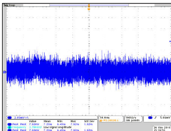
Figure 16: LGA80D-00DADJJ Ripple and Noise - V_o = 0.6V
