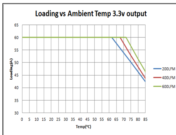
Figure 14: LGA80D-00DADJJ Thermal Derating Curves (Two modules with longitudinal airflow) Vin = 12V Load: Io = 35 to 60A, Vo = 3.3V Fsw = 571kHz
