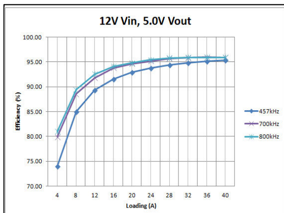
Figure 10: LGA80D-00DADJJ Efficiency Curves @ 25°C, 200LFM
