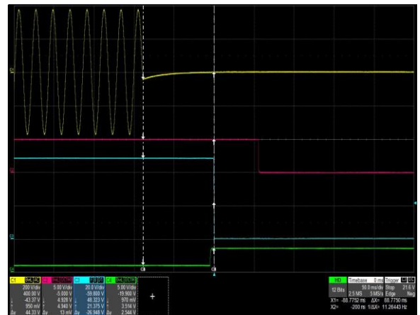
Figure 24: µMP10T-S2W-HUP-00-A Hold-up Time Vin = 264Vac/47Hz Load: I O = 5A I SB = 2A Ch 1: AC Mains Ch 2: V SB Ch 3: V O Ch 4: Global DCOK
