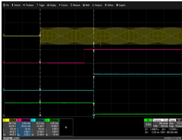
Figure 19: µMP10T-S2Q-S2Q-S2Q-S2Q-S2Q-90-A Turn-on delay via AC mains Vin = 90Vac Load: I O = 41.66A I SB = 2A Ch 1: AC Mains Ch 2: V SB Ch 3: V O Ch 4: Global DCOK
