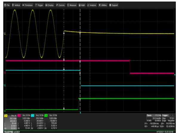
Figure 22: µMP10T-S2Q-S2Q-S2Q-S2Q-S2Q-90-A Hold-up Time via AC mains Vin = 264Vac/47Hz Load: I O = 50A I SB = 2A Ch 1: AC Mains Ch 2: V SB Ch 3: V O Ch 4: Global DCOK
