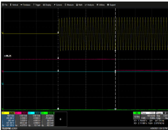
Figure 27: μMP10T-S2Q-S2Q-S2Q-S2Q-S2Q-90-A AC OK Delay - Turn on Vin = 90Vac Load: Io = 41.66A Ch 1: V IN Ch 2: Input AC OK Ch 3: Global DC OK Ch 4: Vo
