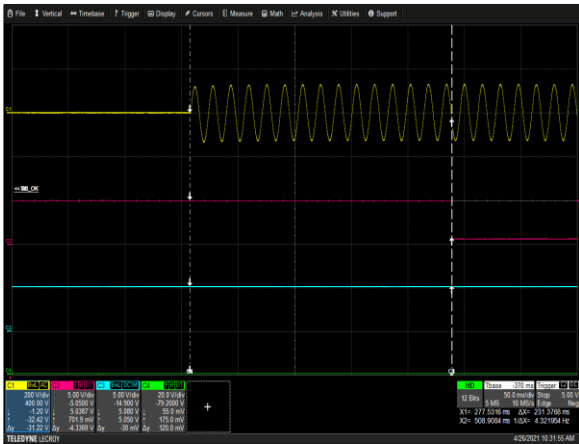
Figure 38: μMP16C-SKQ-SKQ-30-A AC OK Delay - Turn on Vin = 90Vac Load: Io = 41.66A I SB = 0A Turn On Phase = 90° Ch 1: V N Ch 2: Input AC OK Ch 3: Global DC OK Ch 4: V o
