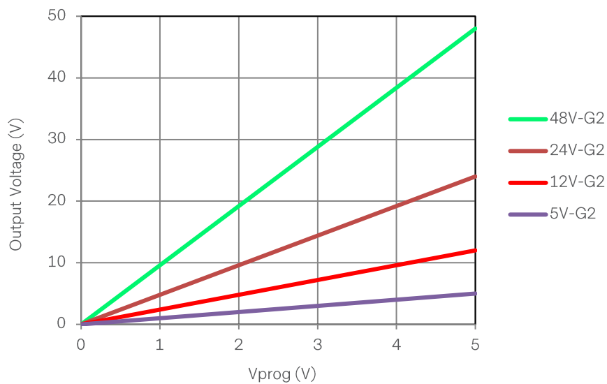
Figure 55 Example of Vprog vs. output Voltage
