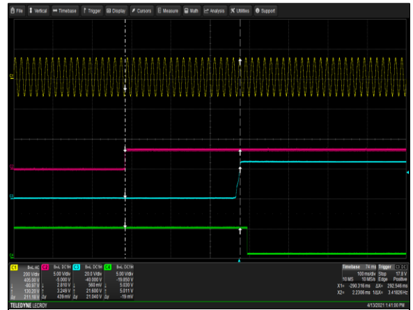
Figure 20: µMP10T-S2Q-S2Q-S2Q-S2Q-S2Q-90-A Turn-on delay via Global inhibit Vin = 90Vac Load: I O = 41.66A I SB = 2A Ch 1: AC Mains Ch 2: Global inhibit Ch 3: V O Ch 4: Global DCOK
