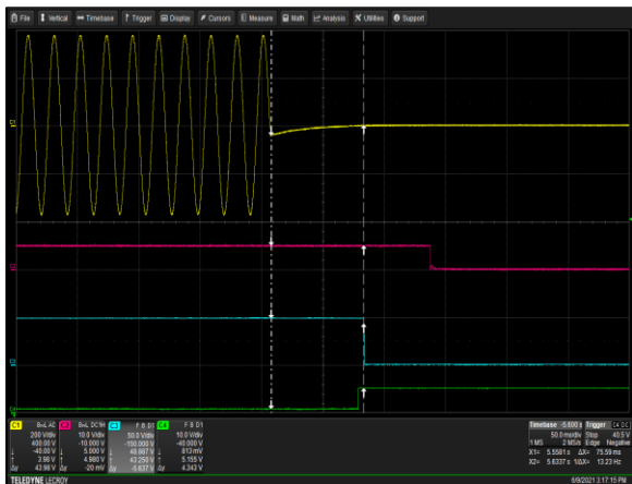
Figure 23: µMP10T-S2W-00-A Hold-up Time Vin = 264Vac/47Hz Load: I O = 5A I SB = 2A Ch 1: AC Mains Ch 2: V SB Ch 3: V O Ch 4: Global DCOK
