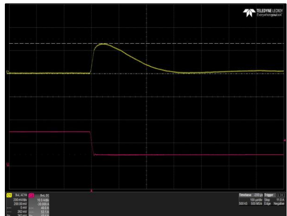
Figure 44: μMP16T-S2L-00-A Transient Response - V_o Deviation 75% to 25% load change, 1A/\mu S slew rate Ch 1: V_o Ch 2: I_o
