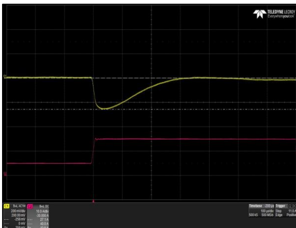
Figure 43: μMP16T-S2L-00-A Transient Response - V_o Deviation 25% to 75% load change, 1A/\mu S slew rate Ch 1: V_o Ch 2: I_o
