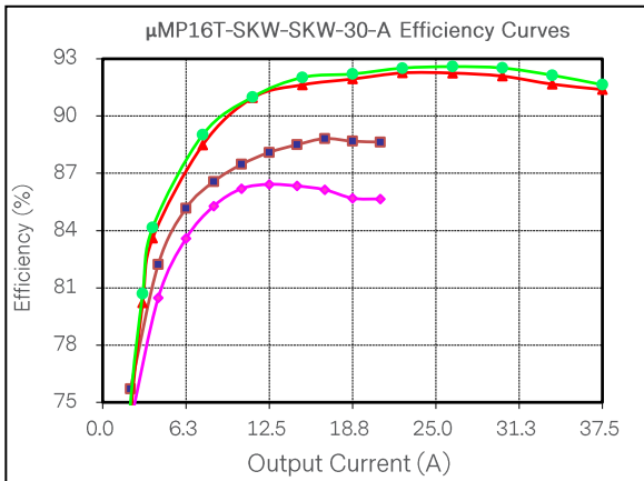
Figure 40: μMP16T-SKW-SKW-30-A Efficiency Curve @ 25°C Loading: I o,main = 10% I o,max increment to 37.5A, I SB = 0A
