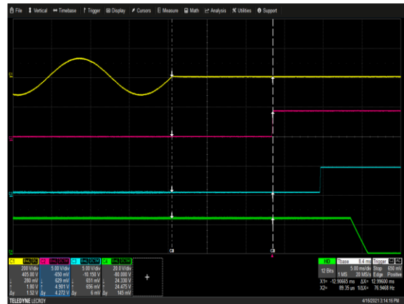
Figure 39: μMP16C-SKQ-SKQ-30-A AC OK Delay - Turn off Vin = 90Vac Load: Io = 41.66A I SB = 0A Turn On Phase = 90° Ch 1: V N Ch 2: Input AC OK Ch 3: Global DC OK Ch 4: V o
