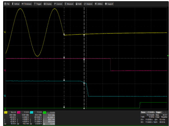
Figure 13: µMP09T-SKQ-S2Q-30-A Hold-up Time Vin = 264Vac/47Hz Load: I O = 41.6A I SB = 2A Ch 1: AC Mains Ch 2: V SB Ch 3: V O Ch 4: Global DCOK
