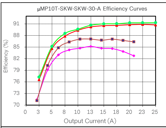
Figure 29: μMP10T-SKW-SKW-30-A Efficiency Curve @ 25°C Loading: I o,main = 10% I o,max increment to 25A, I SB = 0A
