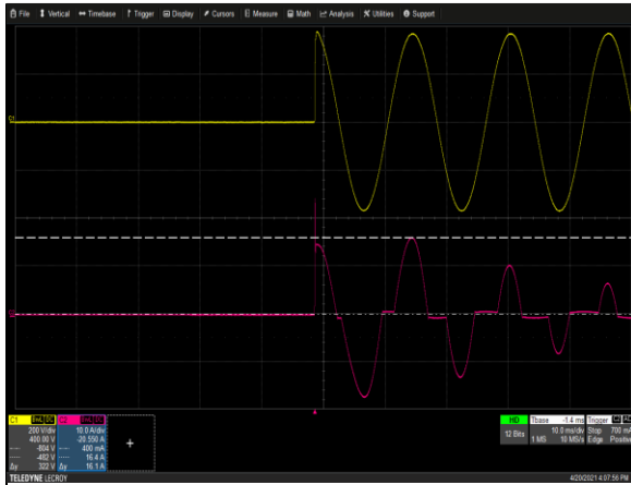
Figure 36: μMP16C-SKQ-SKQ-30-A Start up Inrush Current Vin = 264Vac Load: Io = 75A I SB = 2A Turn On Phase = 90° Ch 1: V N Ch 2: I IN
