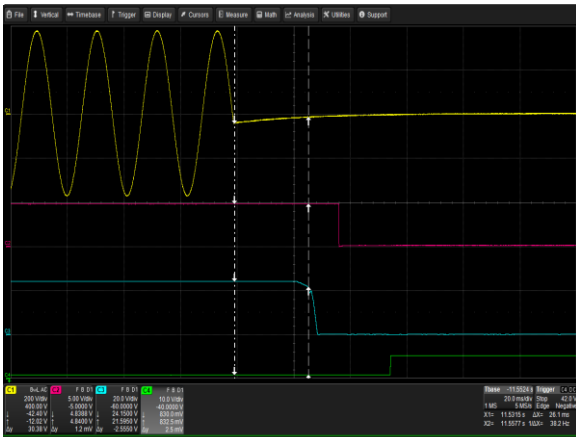
Figure 14: µMP09T-SKQ-00-A Hold-up Time Vin = 264Vac/47Hz Load: I O = 20.83A I SB = 2A Ch 1: AC Mains Ch 2: V SB Ch 3: V O Ch 4: Global DCOK
