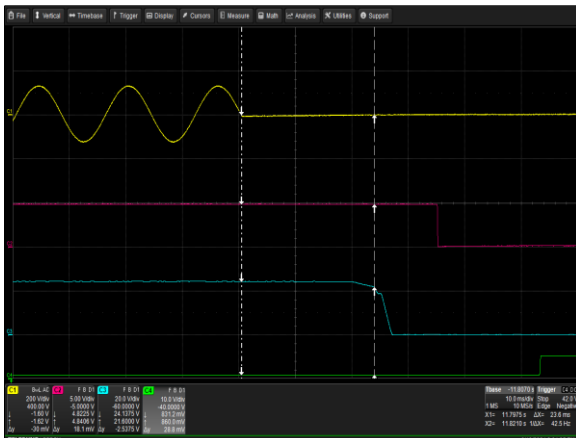
Figure 12: µMP09T-SKQ-S2Q-30-A Hold-up Time Vin = 90Vac/63Hz Load: I O = 23A I SB = 2A Ch 1: AC Mains Ch 2: V SB Ch 3: V O Ch 4: Global DCOK
