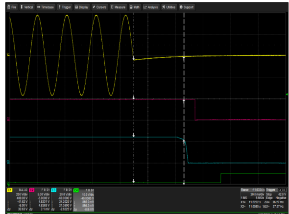
Figure 15: µMP09T-SKQ-HUP-00-A Hold-up Time Vin = 264Vac/47Hz Load: I O = 20.83A I SB = 2A Ch 1: AC Mains Ch 2: V SB Ch 3: V O Ch 4: Global DCOK
