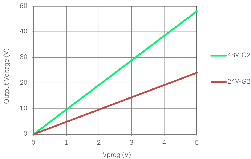
Figure 56 Example of Vprog vs. output Voltage
