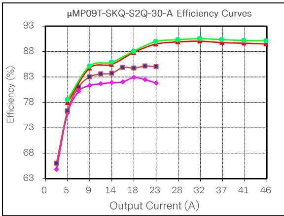
Figure 18: μMP09T-SKQ-S2Q-30-A Efficiency Curve @ 25°C Loading: I O,main = 10% I O,max increment to 45.8A, I SB = 0A
