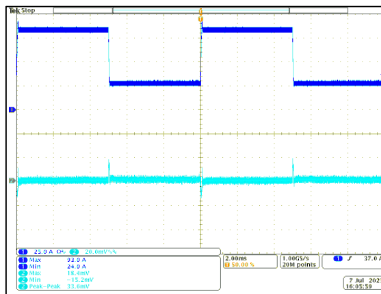
Figure 37: LGA110D-01DADJJ Transient Response - V_O Deviation 25% to 75% to 25% load change, 1A/ \mu S slew rate, V_{in} = 12V_{dc} V_O = 1.0V Ch 1: I_O Ch 2: V_O F_{SW} = 533kHz
