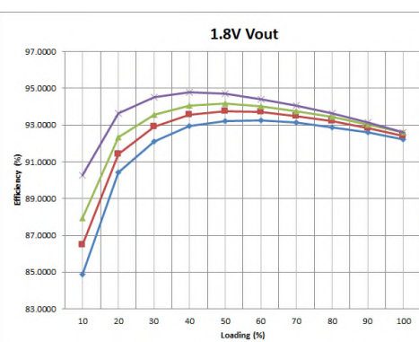
Figure 3: LGA110D-01DADJJB Efficiency Curves at different V_{IN} @ 25°C Loading: I_O = 10% increment to 100A, V_O = 1.8V Frequency=533KHz
