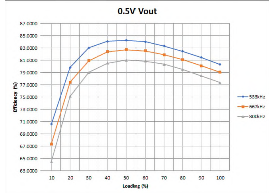
Figure 7: LGA110D-01DADJJB Efficiency Curves at different switching frequency @ 25°C, Vin = 12V Loading: I_O = 10% increment to 110A
