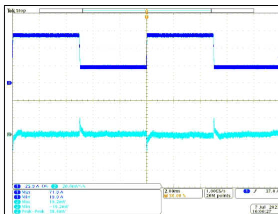
Figure 39: LGA110D-01DADJJ Transient Response - V_O Deviation 25% to 75% to 25% load change, 1A/ \mu S slew rate, V_{in} = 12V_{dc} V_O = 2.5V Ch 1: I_O Ch 2: V_O F_{SW} = 533kHz
