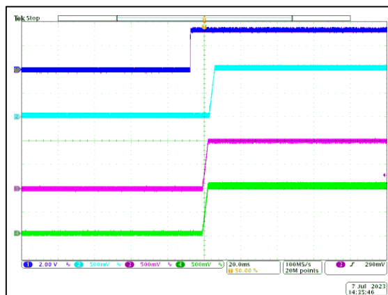
Figure 25: LGA110D-01DADJJB Start Up - V_o = 1V Full Load Ch 1: Enable Ch 2: V_{O1} Ch 3: V_{O2} Ch 4: V_{O3}
