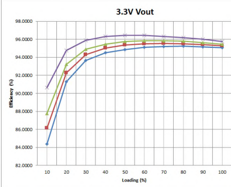
Figure 5: LGA110D-01DADJJB Efficiency Curves at different V_{IN} @ 25°C Loading: I_O = 10% increment to 80A, V_O = 3.3V Frequency=533KHz
