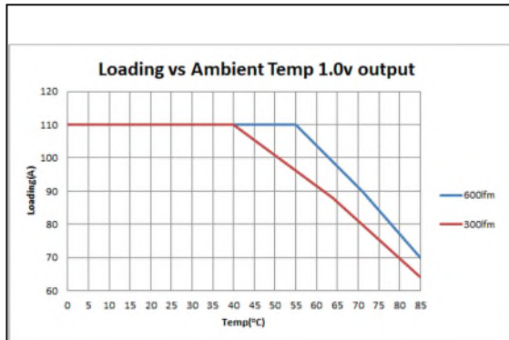
Figure 13: LGA110D-01DADJJB Thermal Derating Curves (Two modules with longitudinal airflow) Vin = 14V Load: I_O = 64 to 110A, V_O = 1.0V F_{SW} = 533kHz
