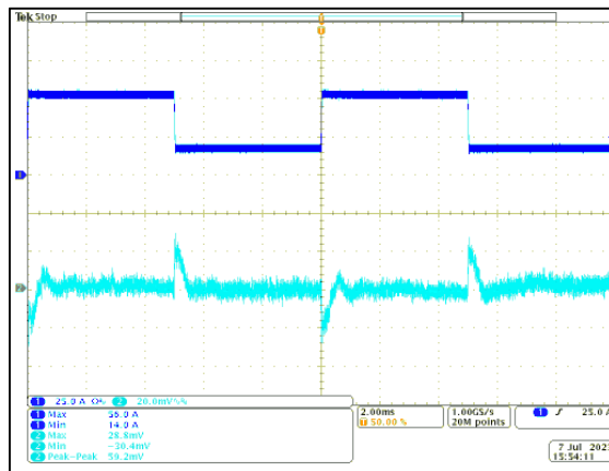
Figure 41: LGA110D-01DADJJ Transient Response - V_O Deviation 25% to 75% to 25% load change, 1A/ \mu S slew rate, V_{in} = 12V_{dc} V_O = 5.0V Ch 1: I_O Ch 2: V_O F_{SW} = 533kHz
