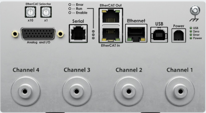
4100T Rear view with four optical channels installed
