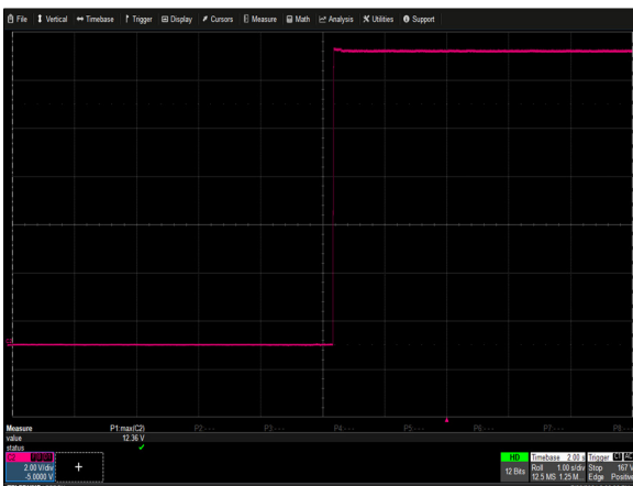
Figure 11: AIF42BAC-01N Output Voltage Startup Characteristic Vin = 230Vac Load: I o = 42A Ch 2: V O
