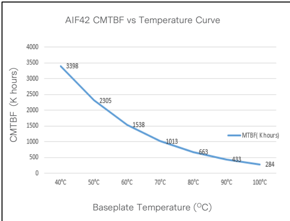
Figure 13: AIF42BAC-01N CMTBF vs Temperature Curve (K hours)
