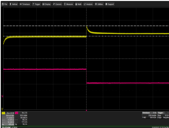
Figure 9: AIF42BAC-01N Transient Response - V O Deviation 100% to 50% load change 1A/μs slew rate Vin = 230Vac Ch 1: V O Ch 2: I O
