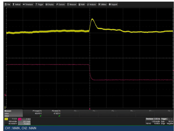
Figure 66: LCM3000W-T Transient Response - Vo Deviation 100% to 50% load change 1A/uS slew rate Vin = 230Vac Ch 1: Vo Ch 2: Io
