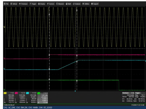
Figure 18: LCM30008-T Turn-on delay via INH_EN Vin = 264Vac Load: Io = 166.7A (18V), Isb = 2A Ch 1: Vin Ch 2: INH_EN Ch 3: Vo Ch 4: G_DCOK_C
