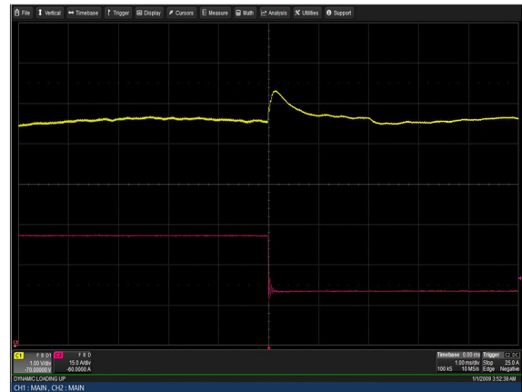
Figure 80: LCM30007-T Transient Response - Vo Deviation 100% to 50% load change 1A/uS slew rate Vin = 230Vac Ch 1: Vo Ch 2: Io
