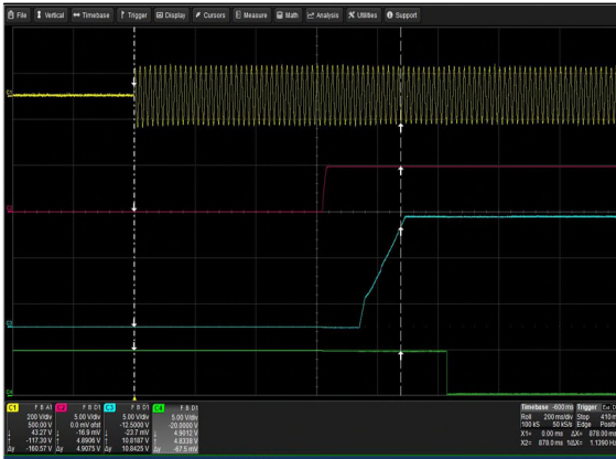
Figure 1: LCM3000L-T Turn-on delay via AC mains Vin = 90Vac Load: Io = 125A (12V), Isb = 2A Ch 1: Vin Ch 2: Vsb Ch 3: Vo Ch 4: G_DCOK_C
