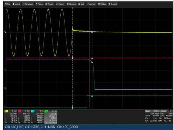
Figure 62: LCM3000W-T Hold-up Time Vin = 264Vac Load: Io = 62.5A (48V), Isb = 2A Ch 1: Vin Ch 2: Vsb Ch 3: Vo Ch 4: G_DCOK_C
