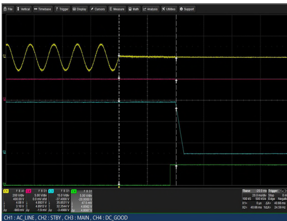
Figure 47: LCM3000U-T Hold-up Time Vin = 90Vac Load: Io = 41.7A (36V), Isb = 2A Ch 1: Vin Ch 2: Vsb Ch 3: Vo Ch 4: G_DCOK_C
