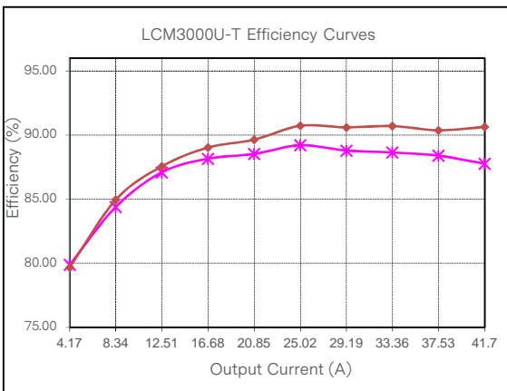
Figure 53: LCM3000U-T Efficiency Curve @ 25°C Loading: I_{o\_min} = 10\%I_{o\_max} increment to 41.7A, I_{sb} = 0A — x — 90Vac — ◆ — 115Vac
