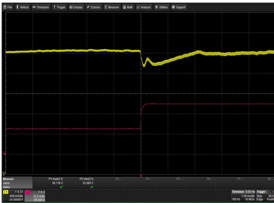
Figure 51: LCM3000U-T Transient Response - V_o Deviation 50% to 100% load change 1A/ \mu s slew rate V_{in} = 230V_{ac} Ch 1: V_o Ch 2: I_o
