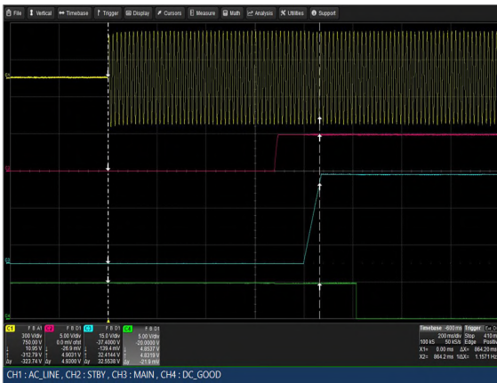
Figure 45: LCM3000U-T Turn-on delay via AC mains Vin = 264Vac Load: Io = 83.3A (36V), Isb = 2A Ch 1: Vin Ch 2: Vsb Ch 3: Vo Ch 4: G_DCOK_C
