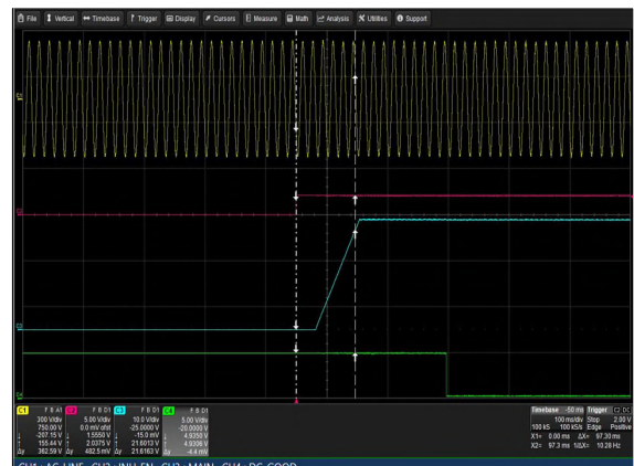
Figure 32: LCM3000Q-T Turn-on delay via INH_EN Vin = 264Vac Load: Io = 125A (24V), Isb = 2A Ch 1: Vin Ch 2: INH_EN Ch 3: Vo Ch 4: G_DCOK_C
