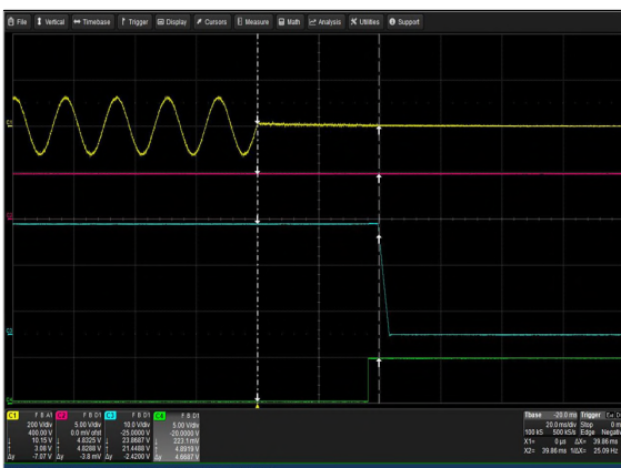
Figure 33: LCM3000Q-T Hold-up Time Vin = 90Vac Load: Io = 62.5A (24V), Isb = 2A Ch 1: Vin Ch 2: Vsb Ch 3: Vo Ch 4: G_DCOK_C
