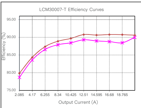
Figure 81: LCM30007-T Efficiency Curve @ 25°C Loading: Io_min = 10%Io_max increment to 20.8A, Isb = 0A
