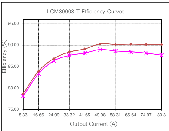
Figure 25: LCM30008-T Efficiency Curve @ 25°C Loading: I_{o\_min} = 10\%I_{o\_max} increment to 83.3A, I_{sb} = 0A — x — 90Vac — ◆ — 115Vac
