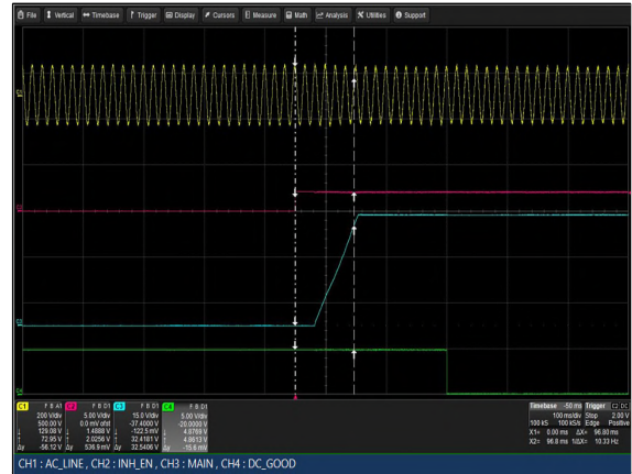
Figure 44: LCM3000U-T Turn-on delay via INH_EN Vin = 90Vac Load: Io = 41.7A (36V), Isb = 2A Ch 1: Vin Ch 2: INH_EN Ch 3: Vo Ch 4: G_DCOK_C
