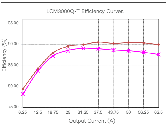
Figure 39: LCM3000Q-T Efficiency Curve @ 25°C Loading: Io_min = 10%Io_max increment to 62.5A, Isb = 0A
