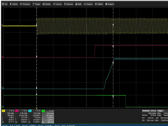
Figure 29: LCM3000Q-T Turn-on delay via AC mains Vin = 90Vac Load: Io = 62.5A (24V), Isb = 2A Ch 1: Vin Ch 2: Vsb Ch 3: Vo Ch 4: G_DCOK_C
