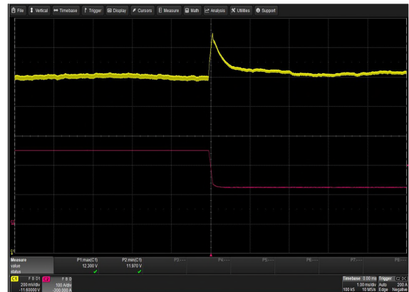
CH1: MAIN, CH2: MAIN Figure 10: LCM3000L-T Transient Response - Vo Deviation 100% to 50% load change 1A/uS slew rate Vin = 230Vac Ch 1: Vo Ch 2: Io
