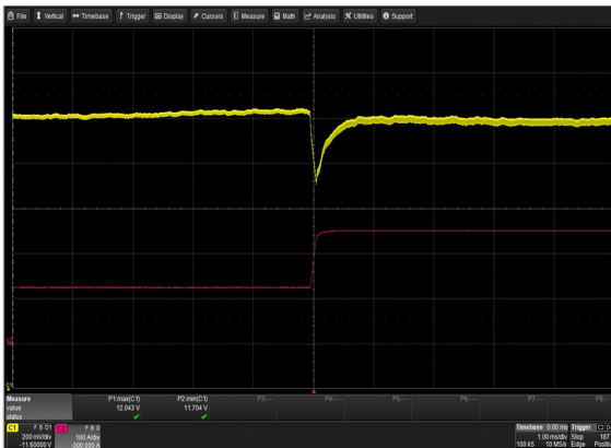
CH1: MAIN, CH2: MAIN Figure 9: LCM3000L-T Transient Response - Vo Deviation 50% to 100% load change 1A/uS slew rate Vin = 230Vac Ch 1: Vo Ch 2: Io
