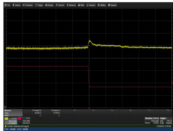
Figure 24: LCM30008-T Transient Response - V_o Deviation 100% to 50% load change 1A/uS slew rate V_{in} = 230V_{ac} Ch 1: V_o Ch 2: I_o
