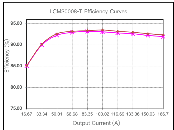
Figure 26: LCM30008-T Efficiency Curve @ 25°C Loading: I_{o\_min} = 10\%I_{o\_max} increment to 166.7A, I_{sb} = 0A — x — 230Vac — ◆ — 264Vac
