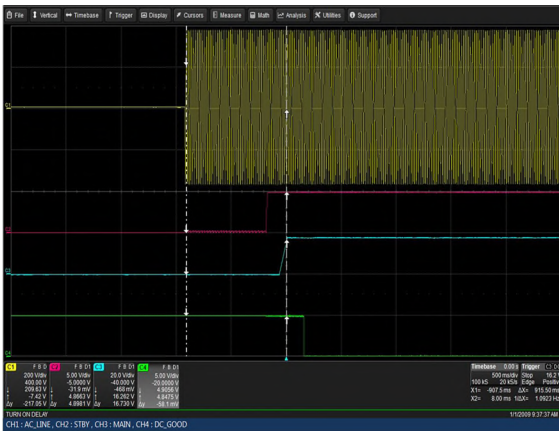
Figure 17: LCM30008-T Turn-on delay via AC mains Vin = 264Vac Load: Io = 166.7A (18V), Isb = 2A Ch 1: Vin Ch 2: Vsb Ch 3: Vo Ch 4: G_DCOK_C
