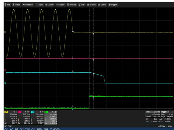
Figure 20: LCM30008-T Hold-up Time Vin = 264Vac Load: Io = 166.7A (18V), Isb = 2A Ch 1: Vin Ch 2: Vsb Ch 3: Vo Ch 4: G_DCOK_C
