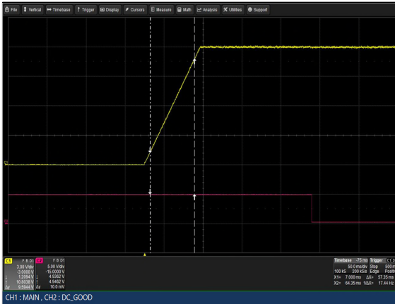
CH1: MAIN, CH2: DC_GOOD Figure 7: LCM3000L-T Output Voltage Startup Vin = 264Vac Load: Io = 125A (12V), Isb = 2A Ch 1: Vo Ch 2: G_DCOK_C
