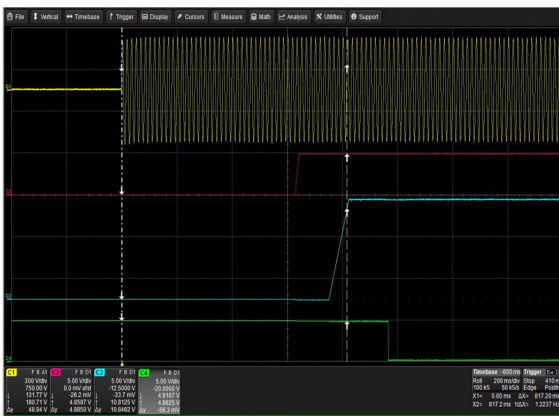
Figure 3: LCM3000L-T Turn-on delay via AC mains Vin = 264Vac Load: Io = 250A (12V), Isb = 2A Ch 1: Vin Ch 2: Vsb Ch 3: Vo Ch 4: G_DCOK_C
