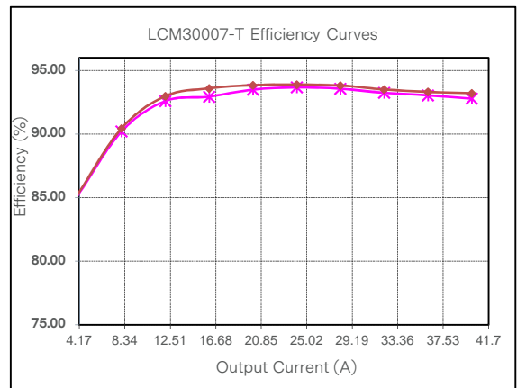
Figure 82: LCM30007-T Efficiency Curve @ 25°C Loading: Io_min = 10%Io_max increment to 41.7A, Isb = 0A
