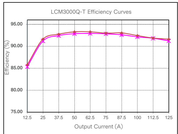
Figure 40: LCM3000Q-T Efficiency Curve @ 25°C Loading: Io_min = 10%Io_max increment to 125A, Isb = 0A
