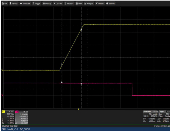
Figure 77: LCM30007-T Output Voltage Startup Vin = 264Vac Load: Io = 41.7A (72V), Isb = 2A Ch 1: Vo Ch 2: G_DCOK_C
