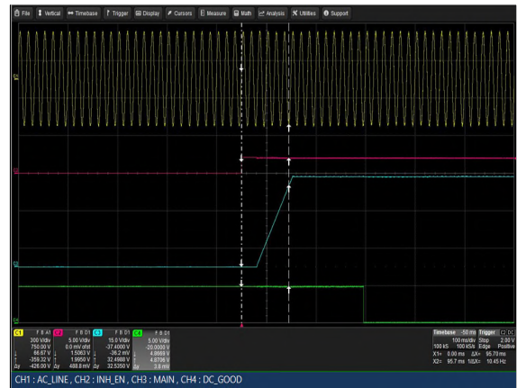
Figure 46: LCM3000U-T Turn-on delay via INH_EN Vin = 264Vac Load: Io = 83.3A (36V), Isb = 2A Ch 1: Vin Ch 2: INH_EN Ch 3: Vo Ch 4: G_DCOK_C
