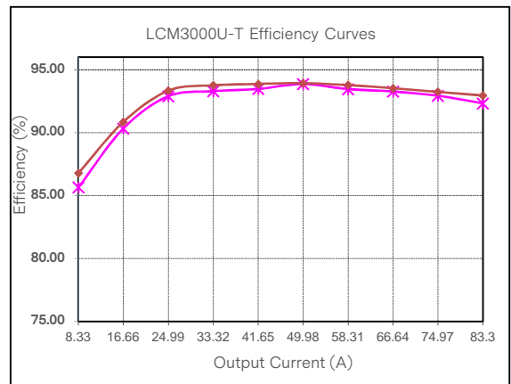
Figure 54: LCM3000U-T Efficiency Curve @ 25°C Loading: I_{o\_min} = 10\%I_{o\_max} increment to 83.3A, I_{sb} = 0A — x — 230Vac — ◆ — 264Vac
