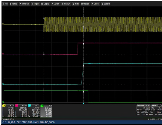
Figure 15: LCM30008-T Turn-on delay via AC mains Vin = 90Vac Load: Io = 83.3A (18V), Isb = 2A Ch 1: Vin Ch 2: Vsb Ch 3: Vo Ch 4: G_DCOK_C
