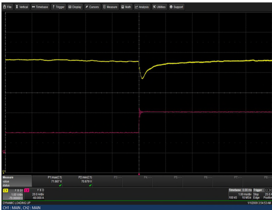
Figure 79: LCM30007-T Transient Response - Vo Deviation 50% to 100% load change 1A/uS slew rate Vin = 230Vac Ch 1: Vo Ch 2: Io
