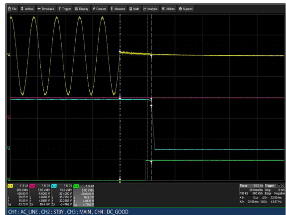
Figure 48: LCM3000U-T Hold-up Time Vin = 264Vac Load: Io = 83.3A (36V), Isb = 2A Ch 1: Vin Ch 2: Vsb Ch 3: Vo Ch 4: G_DCOK_C
