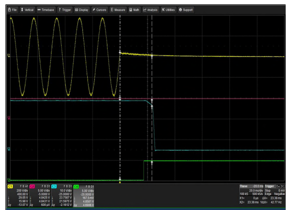
Figure 34: LCM3000Q-T Hold-up Time Vin = 264Vac Load: Io = 125A (24V), Isb = 2A Ch 1: Vin Ch 2: Vsb Ch 3: Vo Ch 4: G_DCOK_C
