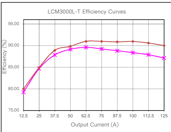
Figure 11: LCM3000L-T Efficiency Curve @ 25°C Loading: Io_min = 10%Io_max increment to 125A, Isb = 0A
