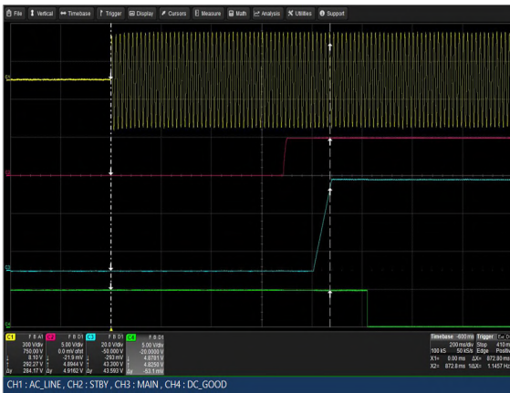
Figure 59: LCM3000W-T Turn-on delay via AC mains Vin = 264Vac Load: Io = 62.5A (48V), Isb = 2A Ch 1: Vin Ch 2: Vsb Ch 3: Vo Ch 4: G_DCOK_C
