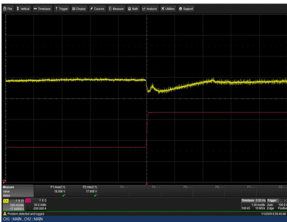
Figure 23: LCM30008-T Transient Response - V_o Deviation 50% to 100% load change 1A/uS slew rate V_{in} = 230V_{ac} Ch 1: V_o Ch 2: I_o
