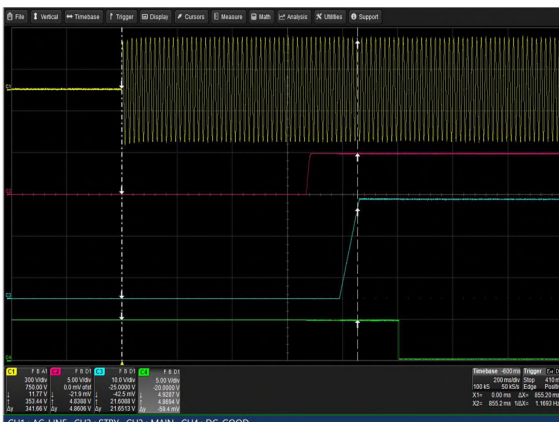
Figure 31: LCM3000Q-T Turn-on delay via AC mains Vin = 264Vac Load: Io = 125A (24V), Isb = 2A Ch 1: Vin Ch 2: Vsb Ch 3: Vo Ch 4: G_DCOK_C
