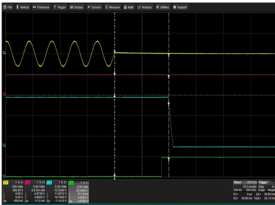
Figure 5: LCM3000L-T Hold-up Time Vin = 90Vac Load: Io = 125A (12V), Isb = 2A Ch 1: Vin Ch 2: Vsb Ch 3: Vo Ch 4: G_DCOK_C
