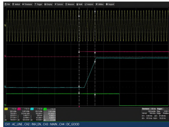
Figure 60: LCM3000W-T Turn-on delay via INH_EN Vin = 264Vac Load: Io = 62.5A (48V), Isb = 2A Ch 1: Vin Ch 2: INH_EN Ch 3: Vo Ch 4: G_DCOK_C
