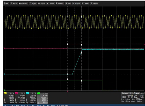
Figure 30: LCM3000Q-T Turn-on delay via INH_EN Vin = 90Vac Load: Io = 62.5A (24V), Isb = 2A Ch 1: Vin Ch 2: INH_EN Ch 3: Vo Ch 4: G_DCOK_C
