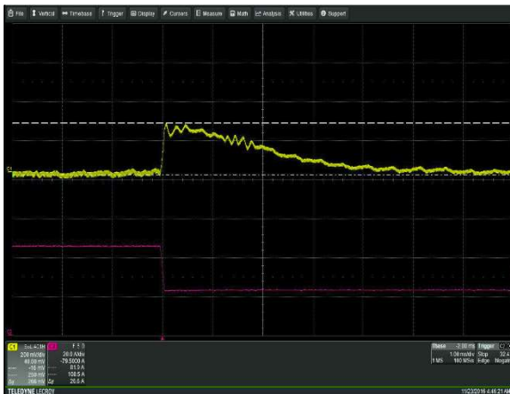
Figure 9: CSU550AP-3 Transient Response - V_O Deviation
