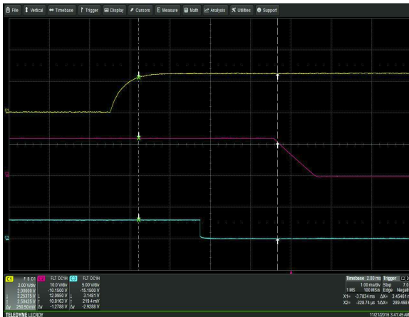
Figure 7: CSU550AP-3 Turn Off Characteristic via PSN
