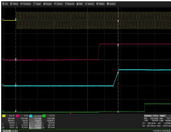
Figure 1: CSU550AP-3 Turn-on delay via AC mains
