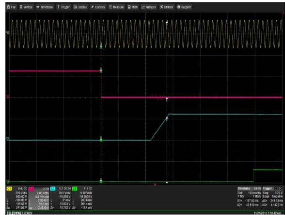
Figure 2: CSU550AP-3 Turn-on delay via PSOn
