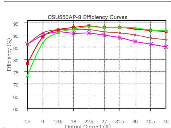
Figure 10: CSU550AP-3 Efficiency Curve @ 25°C
