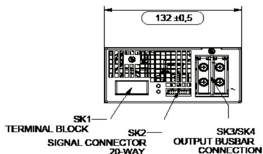
PSU Front View (24V &amp; 48V UNITS)
