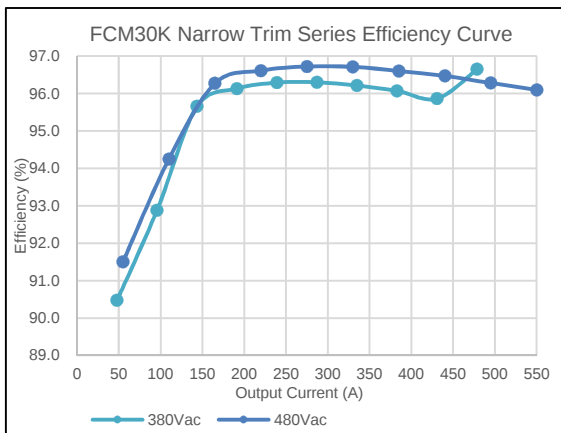
Figure 9: FCM30K Efficiency Curve @ 25°C V_{in} = 380/480 VAC Loading: I_o = 10\% \sim 100\% I_{o,max}
