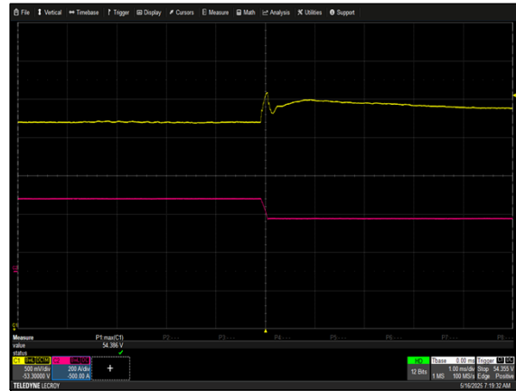
Figure 8: FCM30K Transient Response - Vo Deviation 100% to 50% load change, 1A/uS slew rate V_{in} = 480VAC Ch 1: Vo Ch 2: Io
