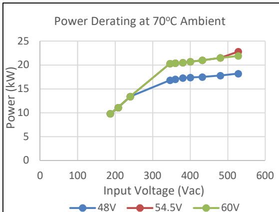
Figure 13: FCM30K Power Derating at 70°C Note: 60°C and 70°C ambient are applicable only for variants without PMI. FCM30KSHNW-PRN and FCM30KSHNW-TRN
