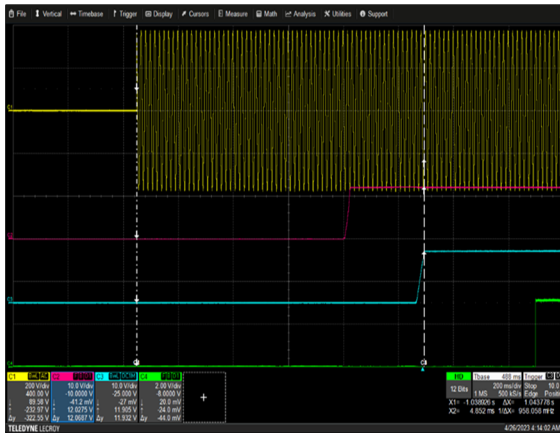
Figure 1: CSU2400AT-3-100 Turn-On Delay via AC Mains V_{in} = 264V_{ac} Load: I_O = 196.7A I_{SB} = 3.5A Ch 1: AC Mains Ch 2: V_{SR} Ch 3: V_O Ch 4: PWOK
