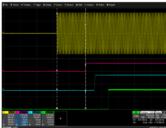
Figure 5: CSU2400AT-3-100 VIN_GOOD Assert Characteristic
