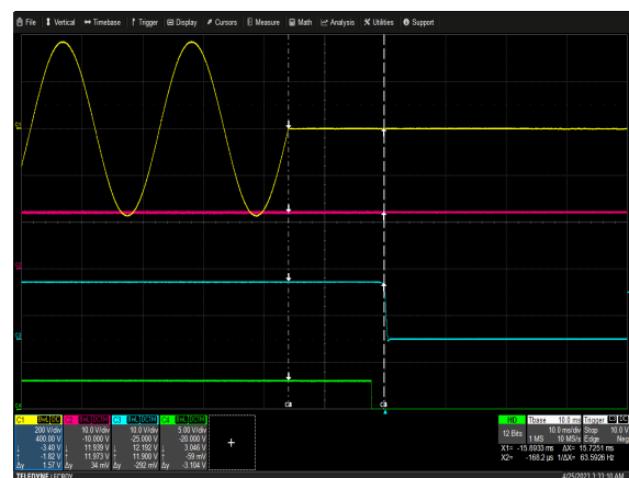
Figure 4: CSU2400T-3-100 Hold-Up Time V_{in} = 264V_{ac} Load: I_o = 196.7A I_{SB} = 3.5A Ch 1: AC Mains Ch 2: V_{SB} Ch 3: V_o Ch 4: PWOK
