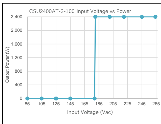
Figure 14: CSU2400AT-3-100 Input Voltage vs Output Power
