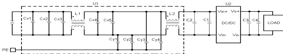
Figure 24 Typical application
