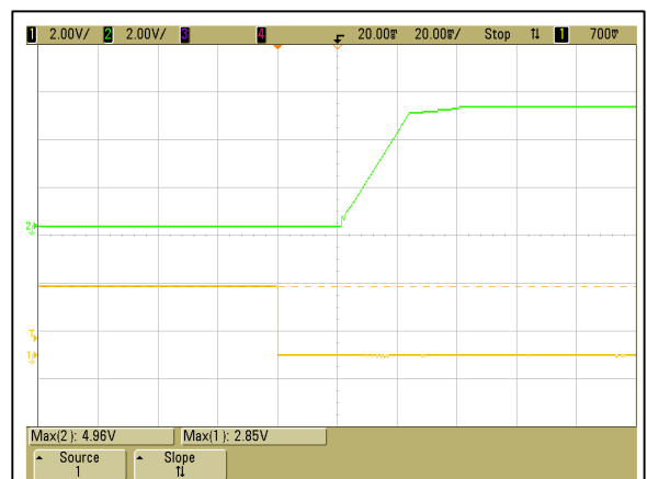
Figure 6: ADO300-48S05 Remote ON Waveform (5mS/div) see figure 12 for test configuration Ch 2: Vo (2V/div) Ch 1: Remote OFF (2V/div)
