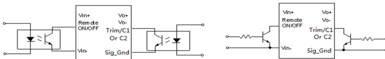
Isolated remote ON/OFF circuit
