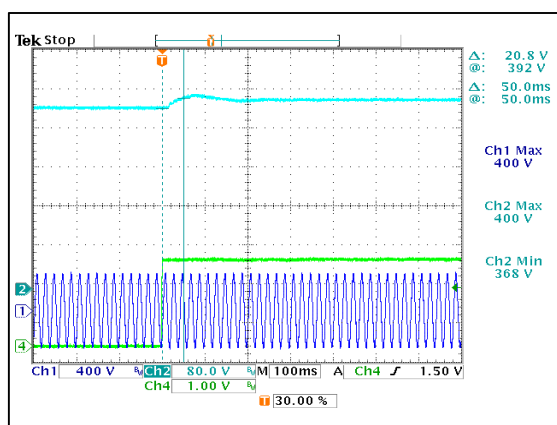
Figure 4: AIH03ZPFC-01L Turn-on delay via PF ENABLE
