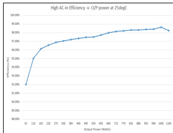
Figure 12: AIH03ZPFC Efficiency Curve @ 25°C — 230Vac/50Hz Loading: P_{O,max} = 1100W 5% increment to P_{O,max}
