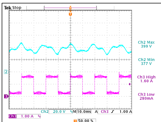
Figure 9: AIH03ZPFC-01L Transient Response - V_o Deviation V_{in} = 90V_{ac} , 10% to 60% load change, Slew rate: 1A/\mu s , C_o = 560\mu F Ch 2: V_o Ch 3: I_o
