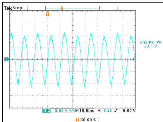
Figure 6: AIH03ZPFC-01L Ripple and Noise Measurement
