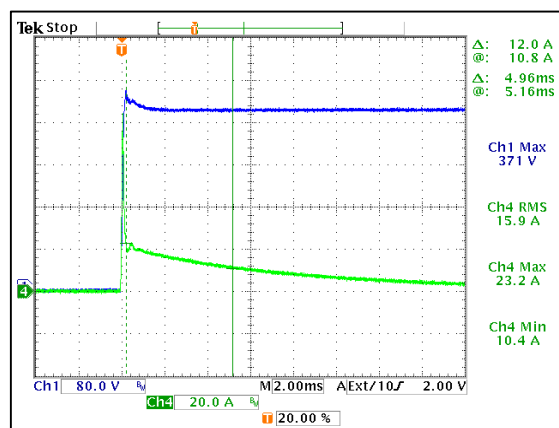
Figure 8: AIH03ZPFC-01L Input Inrush Current V_{in} = 340V_{dc} Load: I_o = 2.8A C_o = 560\mu F Ch 1: V_{in} Ch 4: I_{in}
