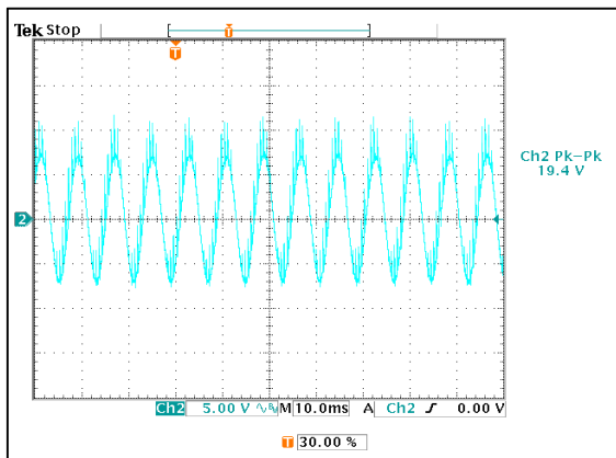
Figure 5: AIH03ZPFC-01L Ripple and Noise Measurement
