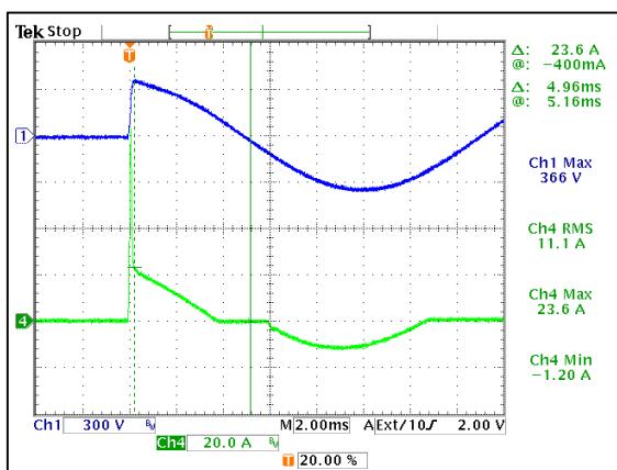
Figure 7: AIH03ZPFC-01L Input Inrush Current V_{in} = 240V_{ac} Load: I_o = 2.8A C_o = 560\mu F Ch 1: V_{in} Ch 4: I_{in}
