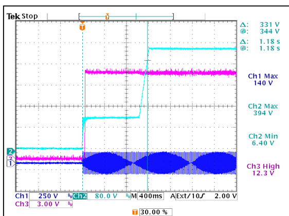
Figure 1: AIH03ZPFC-01L Turn-on Delay via AC mains
