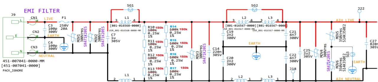
Figure 13: Reference EMI Filter Circuit
