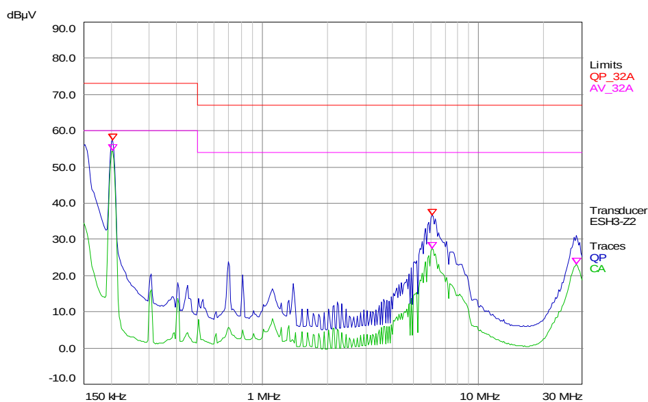
Figure 15: Conducted Emissions
