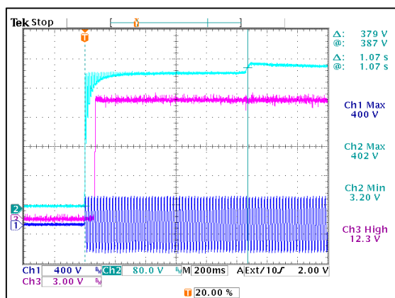
Figure 2: AIH03ZPFC-01L Turn-on Delay via AC mains
