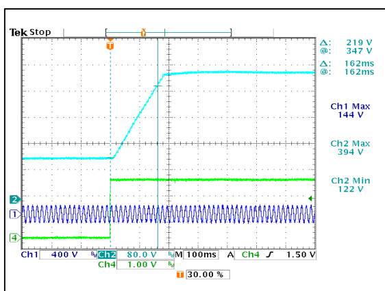
Figure 3: AIH03ZPFC-01L Turn-on delay via PF ENABLE
