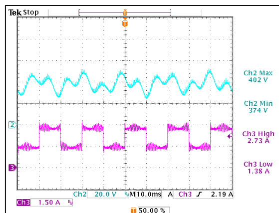
Figure 10: AIH03ZPFC-01L Transient Response - V_o Deviation V_{in} = 90V_{ac} , 50% to 100% load change, Slew rate: 1A/\mu s , C_o = 560\mu F Ch 2: V_o Ch 3: I_o
