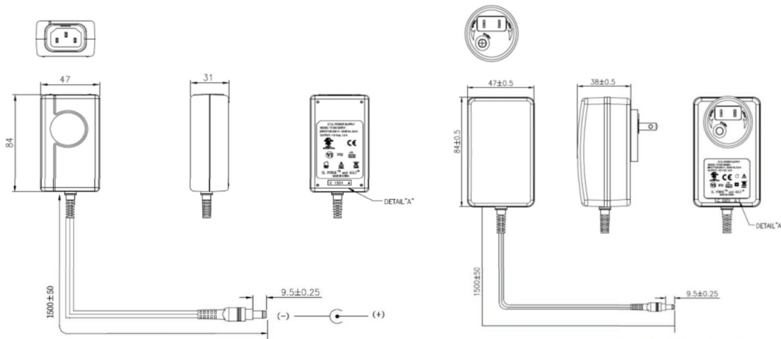
IEC60320 C14 Receptacle, 2.5mm x 5.5mm x 9.5mm Barrel Connector
