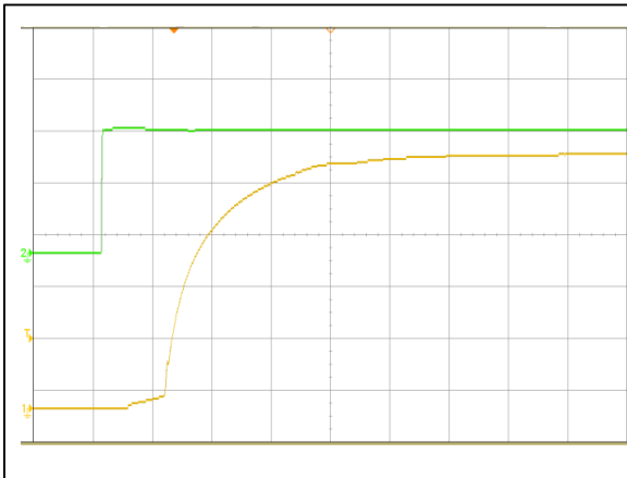
Figure 3: AVD85B-48S05 Output Voltage Startup Characteristic (10mS/div) Ch 1: Vo (1V/div) Ch 2: Vin (20V/div)
