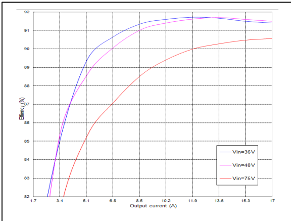
Figure 9: AVD85B-48S05 Efficiency Curves @ 25 °C, 400LFM Loading: Io = 10% increment to 17A
