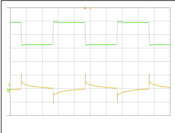
Figure 7: AVD85B-48S05 Transient Response (2mS/div) 50%~75%~50% load change, 0.1A/uS slew rate, Ch 1: Vo (50mV/div) Ch 2: Io (2.5A/div)
