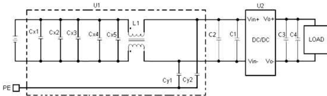
Figure 14. EMC Test Setup
