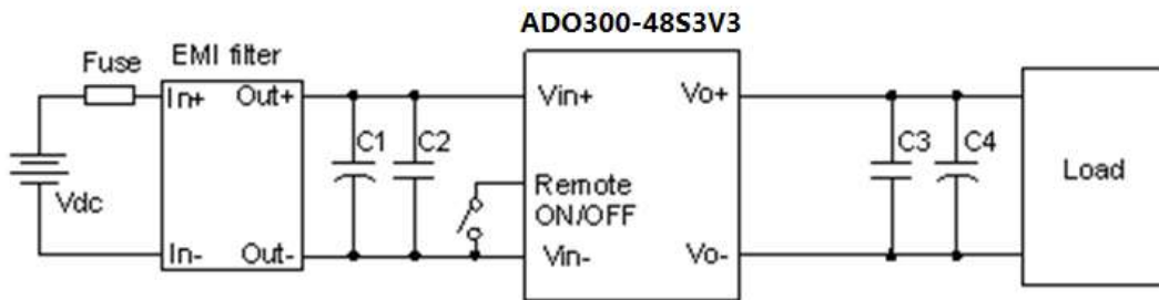
Figure 10. Typical application
