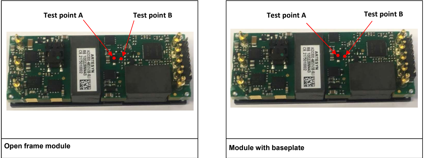
Figure 17. Temperature test point
