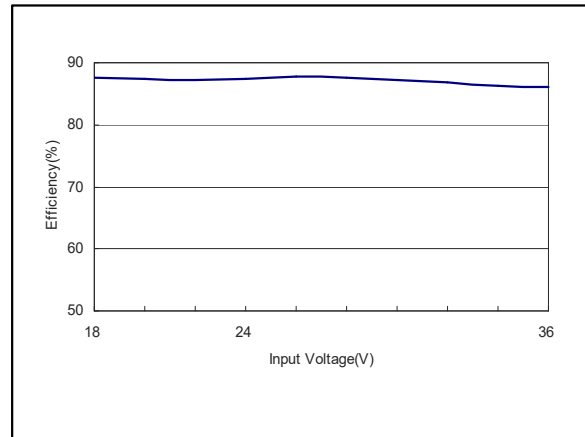
Figure 51: AEE00CC24-M Efficiency Versus Input Voltage Curve Vin = 18 to 36Vdc Load: Io = ±0.333A
