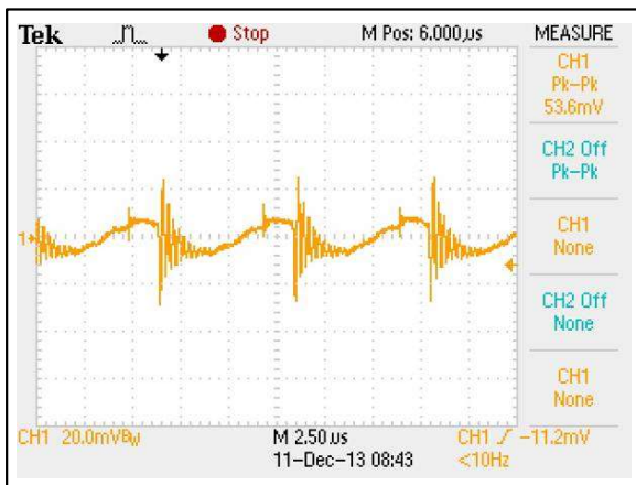
Figure 59: AEE02A48-M Ripple and Noise Measurement Vin = 48Vdc Load: Io = 2A Ch 1: Vo
