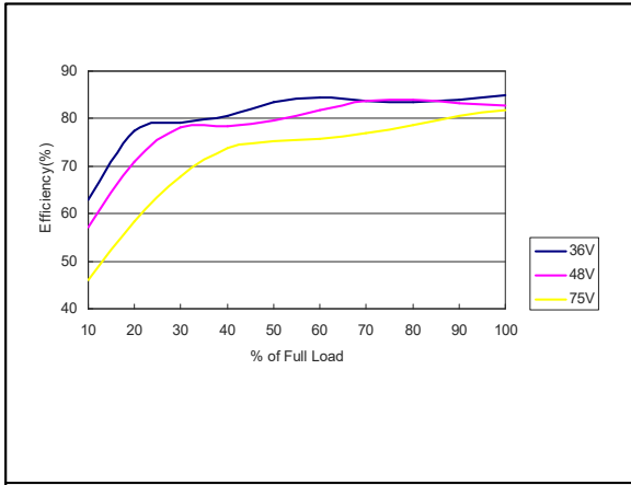
Figure 64: AEE00B48-M Efficiency Versus Output Current Curve Vin = 36 to 75Vdc Load: Io = 0 to 0.835A
