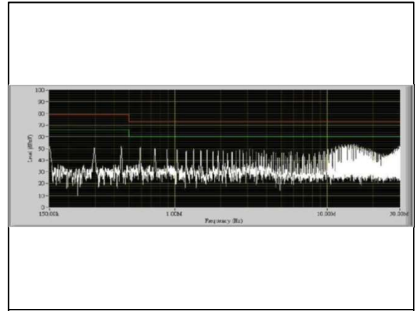
Figure 56: AEE00CC24-M Conduction Emission of EN550122 Class A Vin = 24Vdc Load: Io = ±0.333A
