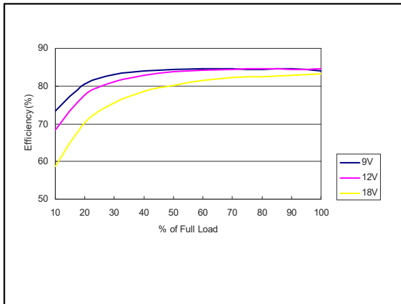
Figure 8: AEE00B12-M Efficiency Versus Output Current Curve Vin = 9 to 18Vdc Load: Io = 0 to 0.835A
