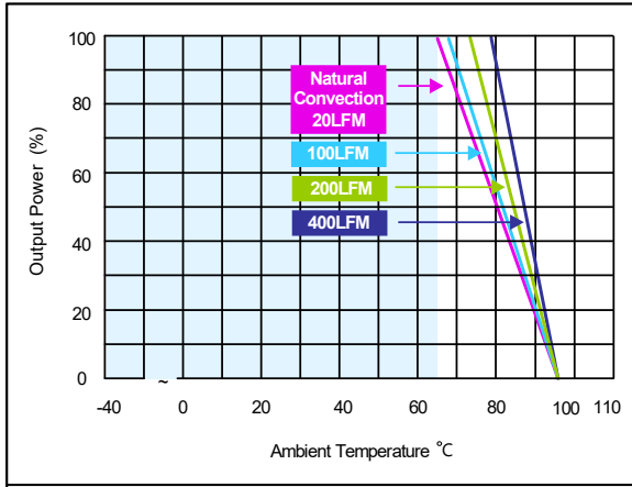
Figure 27: AEE00CC12-M Derating Curves (without heatsink) Vin = 12Vdc Load: Io = 0 to ±0.333A
