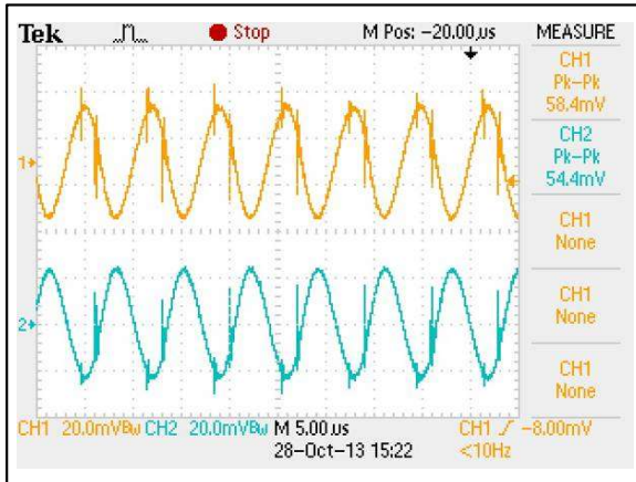
Figure 45: AEE00BB24-M Ripple and Noise Measurement Vin = 24Vdc Load: Io = ±0.417A Ch 1: Vo1 Ch 2: Vo2
