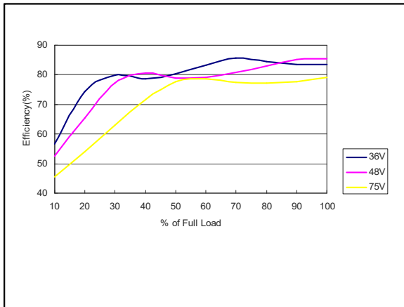
Figure 78: AEE00CC48-M Efficiency Versus Output Current Curve Vin = 36 to 75Vdc Load: Io = 0 to ±0.333A
