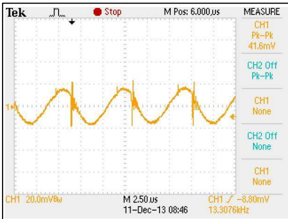
Figure 66: AEE00B48-M Ripple and Noise Measurement Vin = 48Vdc Load: Io = 0.835A Ch 1: Vo
