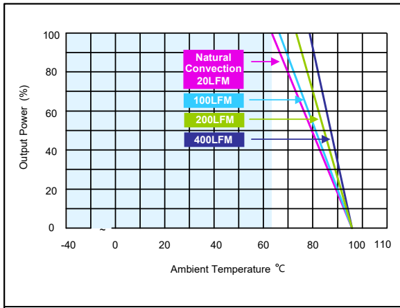
Figure 62: AEE02A48-M Derating Curves (without heatsink) Vin = 48Vdc Load: Io = 0 to 2A
