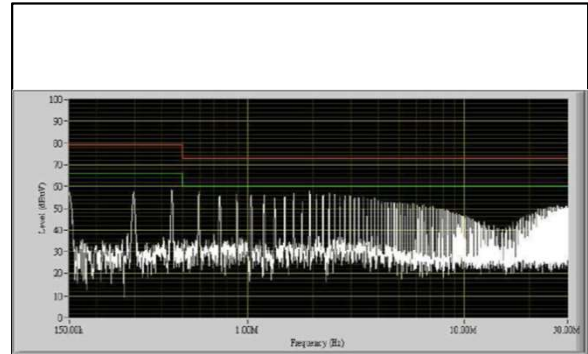
Figure 28: AEE00CC12-M Conduction Emission of EN550122 Class A Vin = 12Vdc Load: Io = ±0.333A
