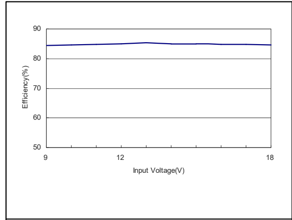
Figure 16: AEE00BB12-M Efficiency Versus Input Voltage Curve Vin = 9 to 18Vdc Load: Io = ±0.417A
