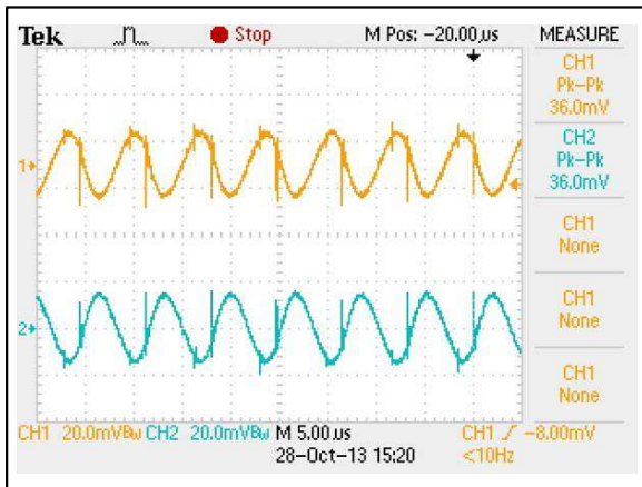
Figure 52: AEE00CC24-M Ripple and Noise Measurement Vin = 24Vdc Load: Io = ±0.333A Ch 1: Vo1 Ch 2: Vo2
