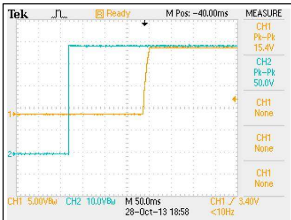
Figure 82: AEE00CC48-M Output Voltage Startup Characteristic by Vin Vin = 48Vdc Load: Io = ±0.333A Ch 1: Vo1 Ch 2: Vin
