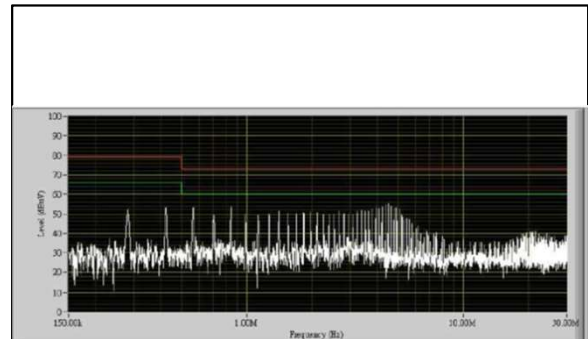
Figure 84: AEE00CC48-M Conduction Emission of EN550122 Class A Vin = 48Vdc Load: Io = ±0.333A
