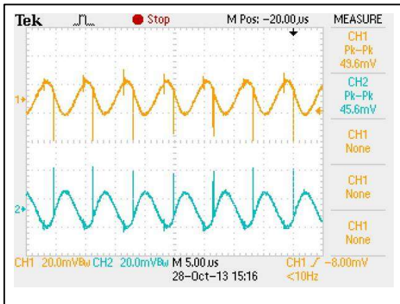
Figure 24: AEE00CC12-M Ripple and Noise Measurement Vin = 12Vdc Load: Io = ±0.333A Ch 1: Vo1 Ch 2: Vo2
