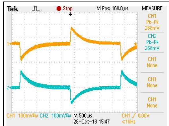
Figure 53: AEE00CC24-M Transient Response Vin = 24Vdc Load: Io = 100% to 75% load change Ch 1: Vo1 Ch 2: Vo2
