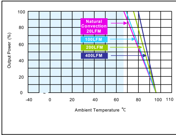
Figure 55: AEE00CC24-M Derating Curves (without heatsink) Vin = 24Vdc Load: Io = 0 to ±0.333A
