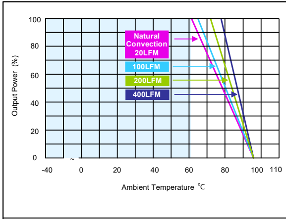
Figure 6: AEE01A12-M Derating Curves (without heatsink) Vin = 12Vdc Load: Io = 0 to 1.6A
