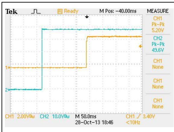
Figure 61: AEE02A48-M Output Voltage Startup Characteristic by Vin Vin = 48Vdc Load: Io = 2A Ch 1: Vo Ch 2: Vin
