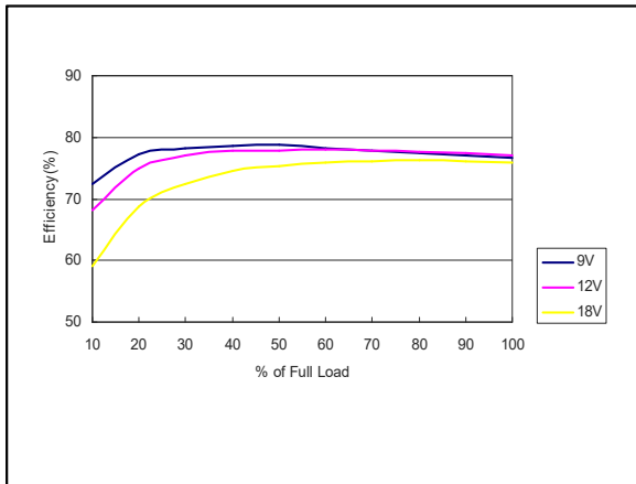
Figure 1: AEE01A12-M Efficiency Versus Output Current Curve Vin = 9 to 18Vdc Load: Io = 0 to 1.6A
