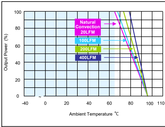
Figure 76: AEE00BB48-M Derating Curves (without heatsink) Vin = 48Vdc Load: Io = 0 to ±0.417A
