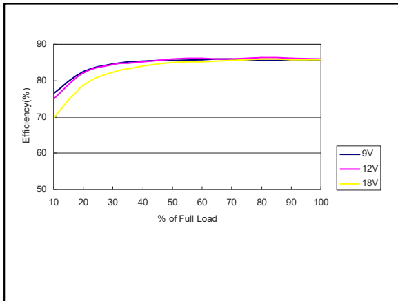
Figure 22: AEE00CC12-M Efficiency Versus Output Current Curve Vin = 9 to 18Vdc Load: Io = 0 to ±0.333A
