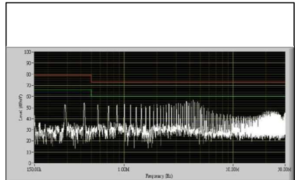
Figure 77: AEE00BB48-M Conduction Emission of EN550122 Class A Vin = 48Vdc Load: Io = ±0.417A
