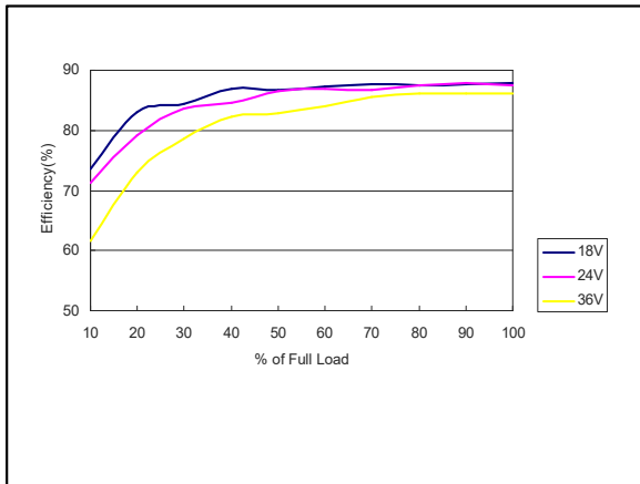
Figure 50: AEE00CC24-M Efficiency Versus Output Current Curve Vin = 18 to 36Vdc Load: Io = 0 to ±0.333A
