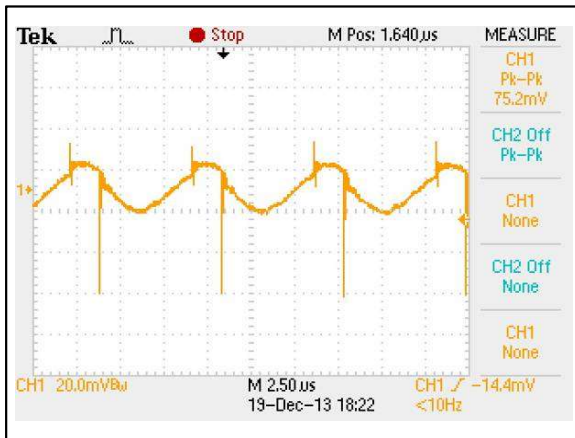
Figure 10: AEE00B12-M Ripple and Noise Measurement Vin = 12Vdc Load: Io = 0.835A Ch 1: Vo
