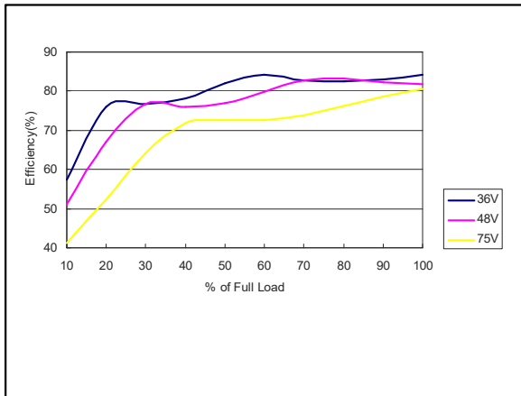
Figure 71: AEE00BB48-M Efficiency Versus Output Current Curve Vin = 36 to 75Vdc Load: Io = 0 to ±0.417A
