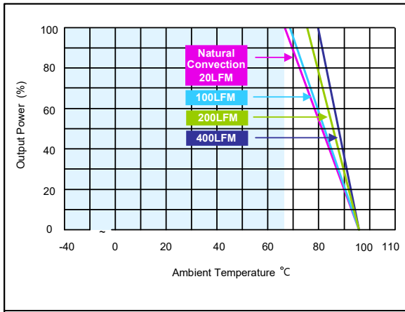
Figure 83: AEE00CC48-M Derating Curves (without heatsink) Vin = 48Vdc Load: Io = 0 to ±0.333A
