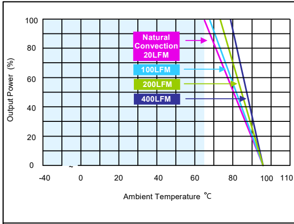
Figure 69: AEE00B48-M Derating Curves (without heatsink) Vin = 48Vdc Load: Io = 0 to 0.835A
