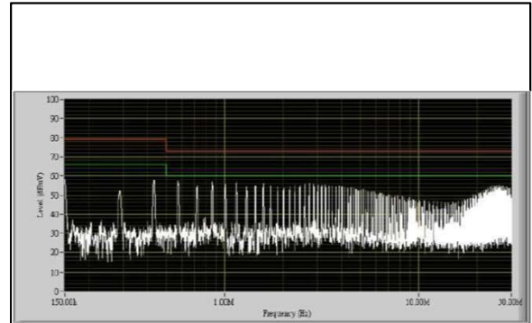
Figure 14: AEE00B12-M Conduction Emission of EN550122 Class A Vin = 12Vdc Load: Io = 0.835A
