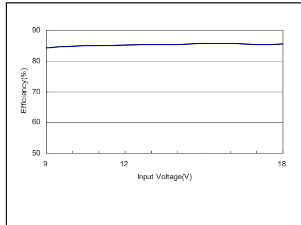
Figure 23: AEE00CC12-M Efficiency Versus Input Voltage Curve Vin = 9 to 18Vdc Load: Io = ±0.333A
