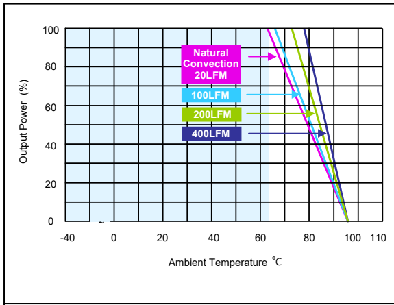
Figure 20: AEE00BB12-M Derating Curves (without heatsink) Vin = 12Vdc Load: Io = 0 to ±0.417A
