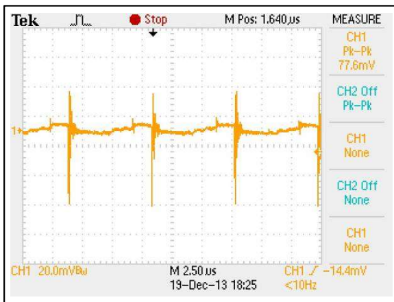
Figure 31: AEE02A24-M Ripple and Noise Measurement Vin = 24Vdc Load: Io = 2A Ch 1: Vo
