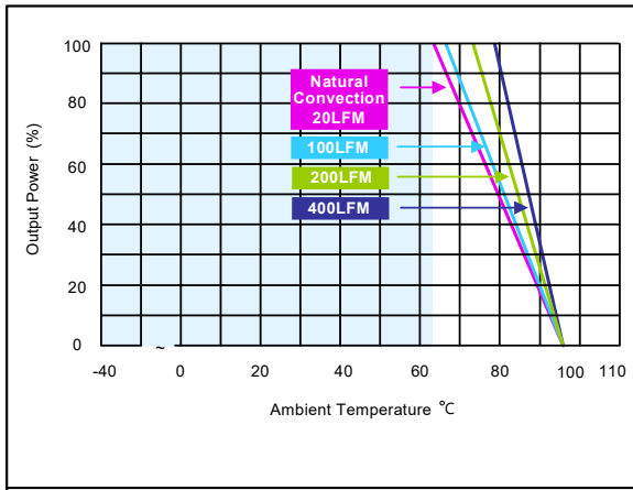
Figure 34: AEE02A24-M Derating Curves (without heatsink) Vin = 24Vdc Load: Io = 0 to 2A
