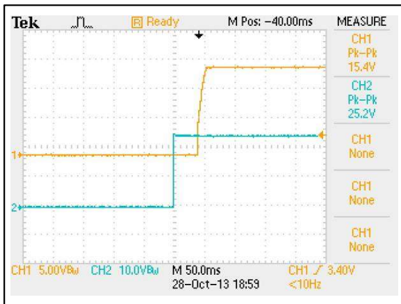
Figure 54: AEE00CC24-M Output Voltage Startup Characteristic by Vin Vin = 24Vdc Load: Io = ±0.333A Ch 1: Vo1 Ch 2: Vin
