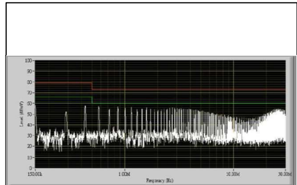
Figure 21: AEE00BB12-M Conduction Emission of EN550122 Class A Vin = 12Vdc Load: Io = ±0.417A
