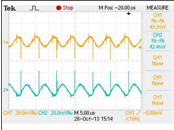
Figure 17: AEE00BB12-M Ripple and Noise Measurement Vin = 12Vdc Load: Io = ±0.417A Ch 1: Vo1 Ch 2: Vo2
