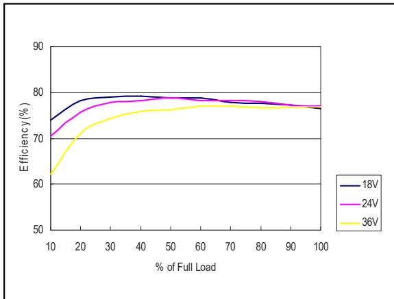
Figure 29: AEE02A24-M Efficiency Versus Output Current Curve Vin = 18 to 36Vdc Load: Io = 0 to 2A
