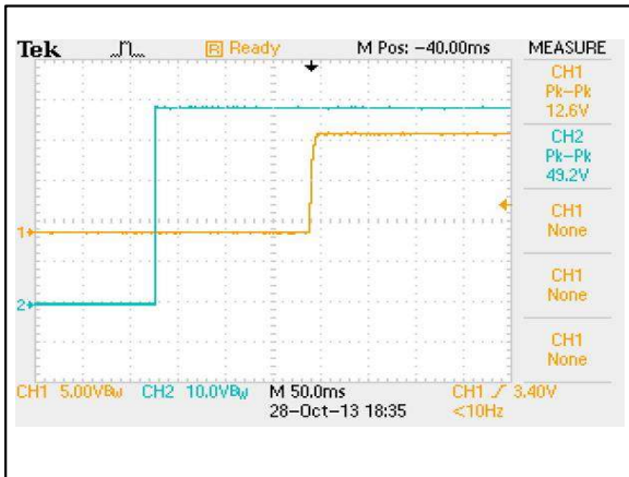
Figure 68: AEE00B48-M Output Voltage Startup Characteristic by Vin Vin = 48Vdc Load: Io = 0.835A Ch 1: Vo Ch 2: Vin
