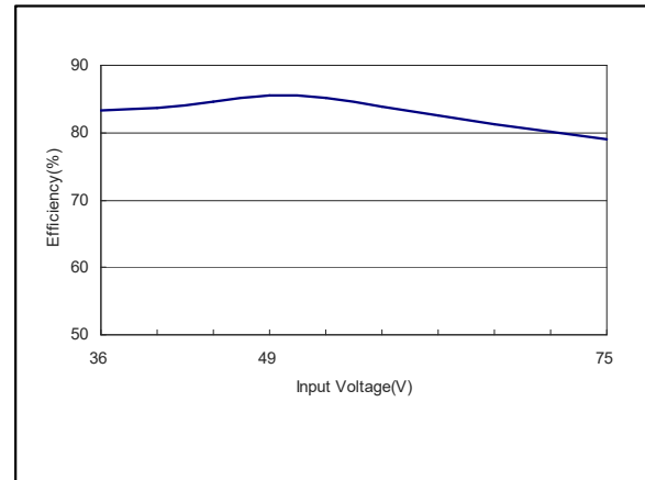
Figure 79: AEE00CC48-M Efficiency Versus Input Voltage Curve Vin = 36 to 75Vdc Load: Io = ±0.333A
