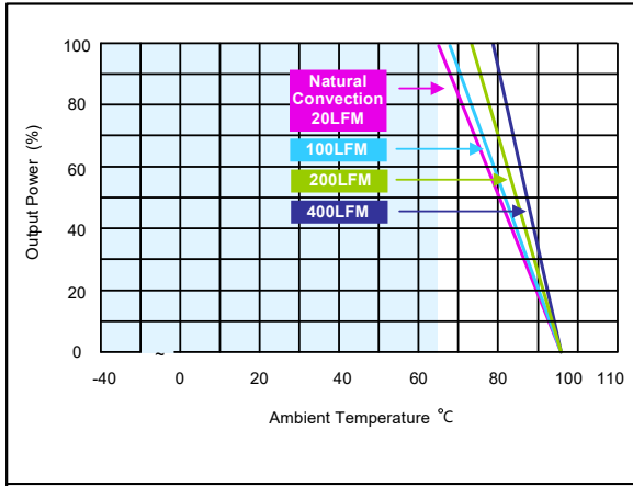
Figure 48: AEE00BB24-M Derating Curves (without heatsink) Vin = 24Vdc Load: Io = 0 to ±0.417A
