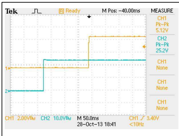
Figure 33: AEE02A24-M Output Voltage Startup Characteristic by Vin Vin = 24Vdc Load: Io = 2A Ch 1: Vo Ch 2: Vin
