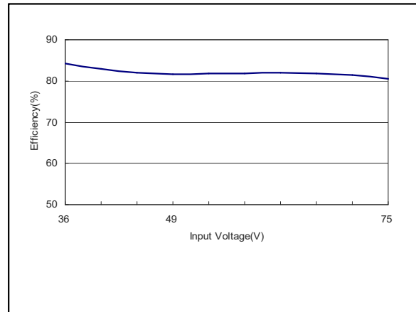
Figure 72: AEE00BB48-M Efficiency Versus Input Voltage Curve Vin = 36 to 75Vdc Load: Io = ±0.417A
