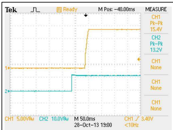
Figure 26: AEE00CC12-M Output Voltage Startup Characteristic by Vin Vin = 12Vdc Load: Io = ±0.333A Ch 1: Vo1 Ch 2: Vin
