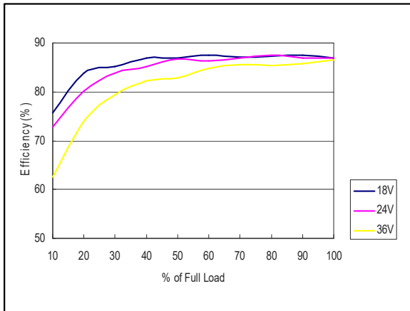
Figure 43: AEE00BB24-M Efficiency Versus Output Current Curve Vin = 18 to 36Vdc Load: Io = 0 to ±0.417A
