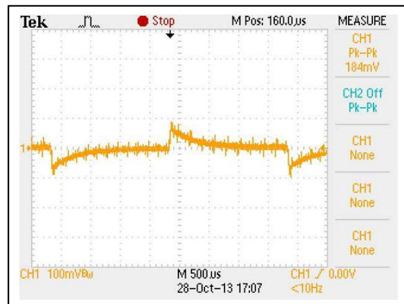
Figure 60: AEE02A48-M Transient Response Vin = 48Vdc Load: Io = 100% to 75% load change Ch 1: Vo
