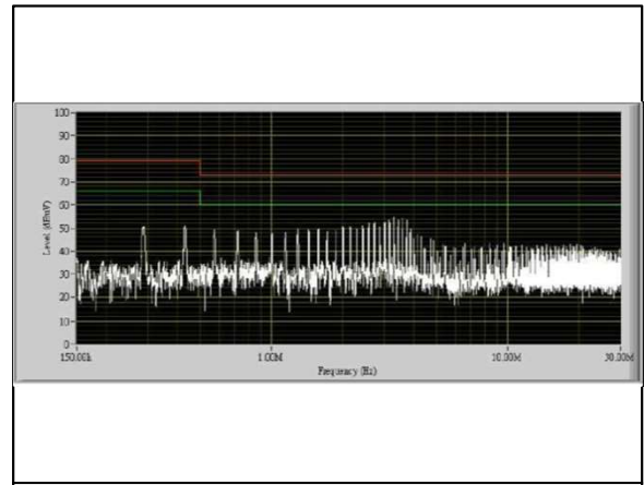
Figure 63: AEE02A48-M Conduction Emission of EN550122 Class A Vin = 48Vdc Load: Io = 2A
