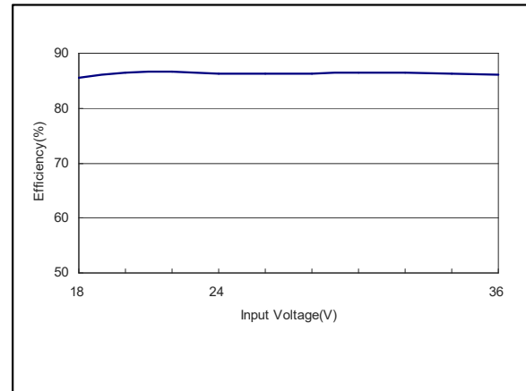
Figure 44: AEE00BB24-M Efficiency Versus Input Voltage Curve Vin = 18 to 36Vdc Load: Io = ±0.417A
