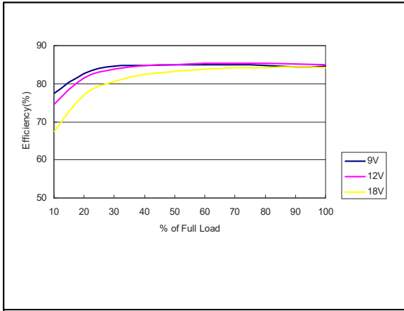
Figure 15: AEE00BB12-M Efficiency Versus Output Current Curve Vin = 9 to 18Vdc Load: Io = 0 to ±0.417A
