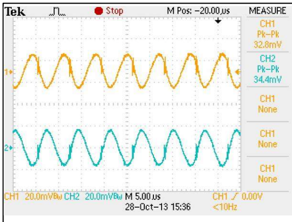
Figure 80: AEE00CC48-M Ripple and Noise Measurement Vin = 48Vdc Load: Io = ±0.333A Ch 1: Vo1 Ch 2: Vo2
