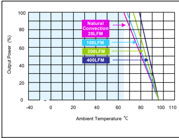
Figure 41: AEE00B24-M Derating Curves (without heatsink) Vin = 24Vdc Load: Io = 0 to 0.835A
