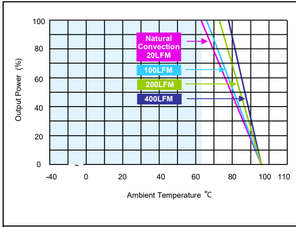
Figure 13: AEE00B12-M Derating Curves (without heatsink) Vin = 12Vdc Load: Io = 0 to 0.835A
