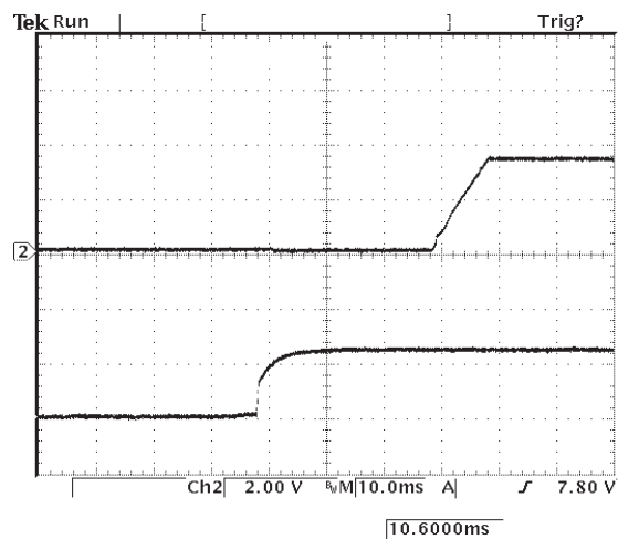
Figure 6: Typical Power-up Characteristic (Channel 1: V_{in} , Channel 2: V_o )
